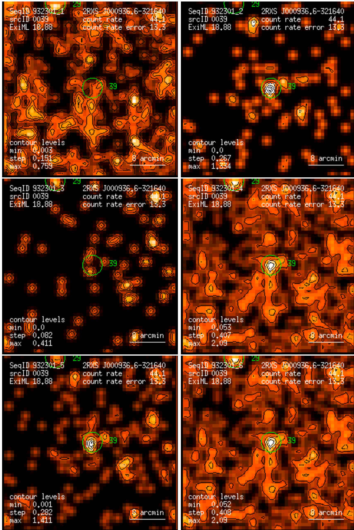
Figure 39: RASS 932301: detection 0039: band rate images, Gaussian filter: (1) PSPC channels 11 – 41, (2) 52 – 90, (3) 91 – 201, (4) 11 – 235, (5) 52 – 201, (6) 11 – 201. Broad band rates in counts/ks. Band rate contour levels in counts/ks/arcmin 2 .
