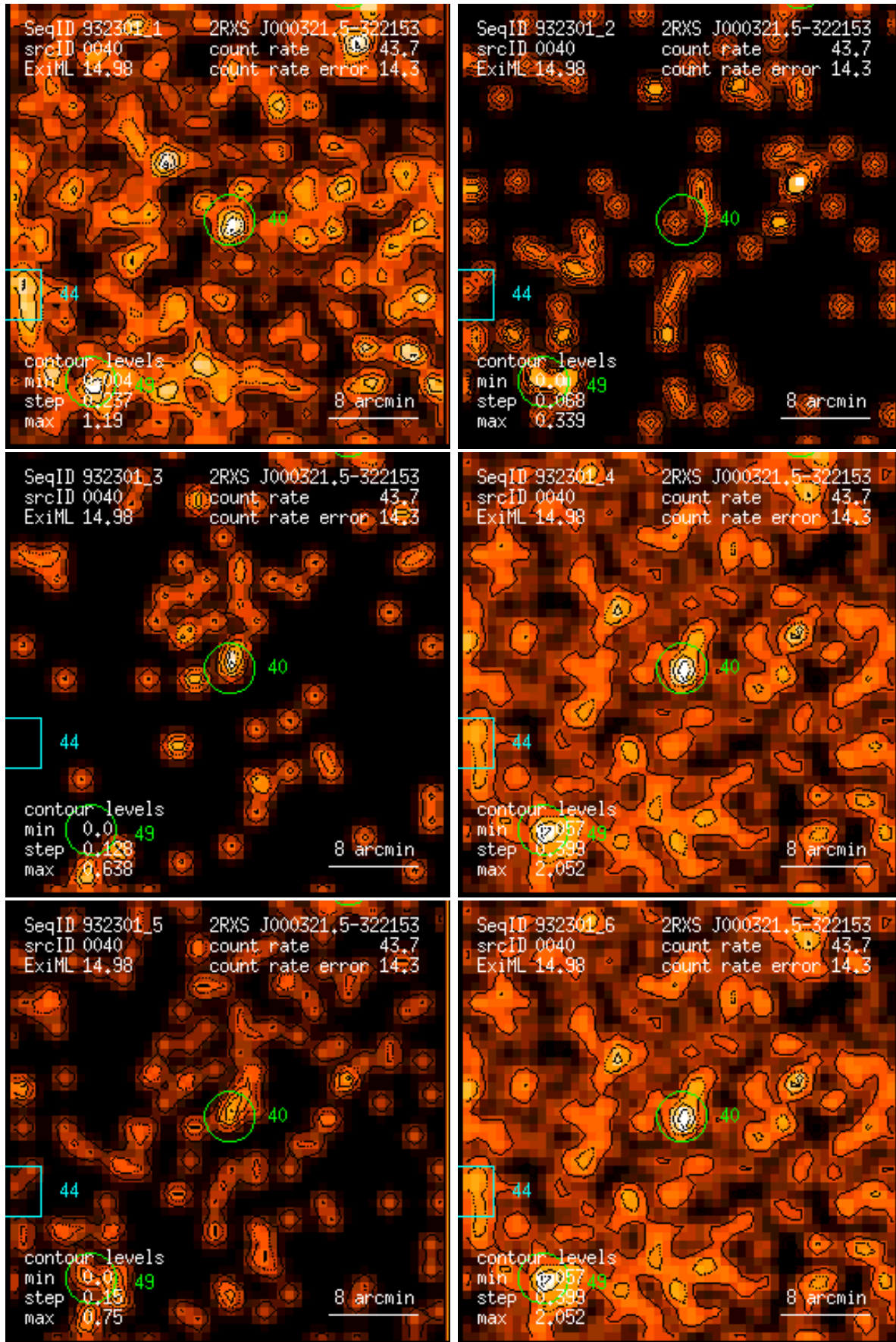
Figure 40: RASS 932301: detection 0040: band rate images, Gaussian filter: (1) PSPC channels 11 – 41, (2) 52 – 90, (3) 91 – 201, (4) 11 – 235, (5) 52 – 201, (6) 11 – 201. Broad band rates in counts/ks. Band rate contour levels in counts/ks/arcmin 2 .
