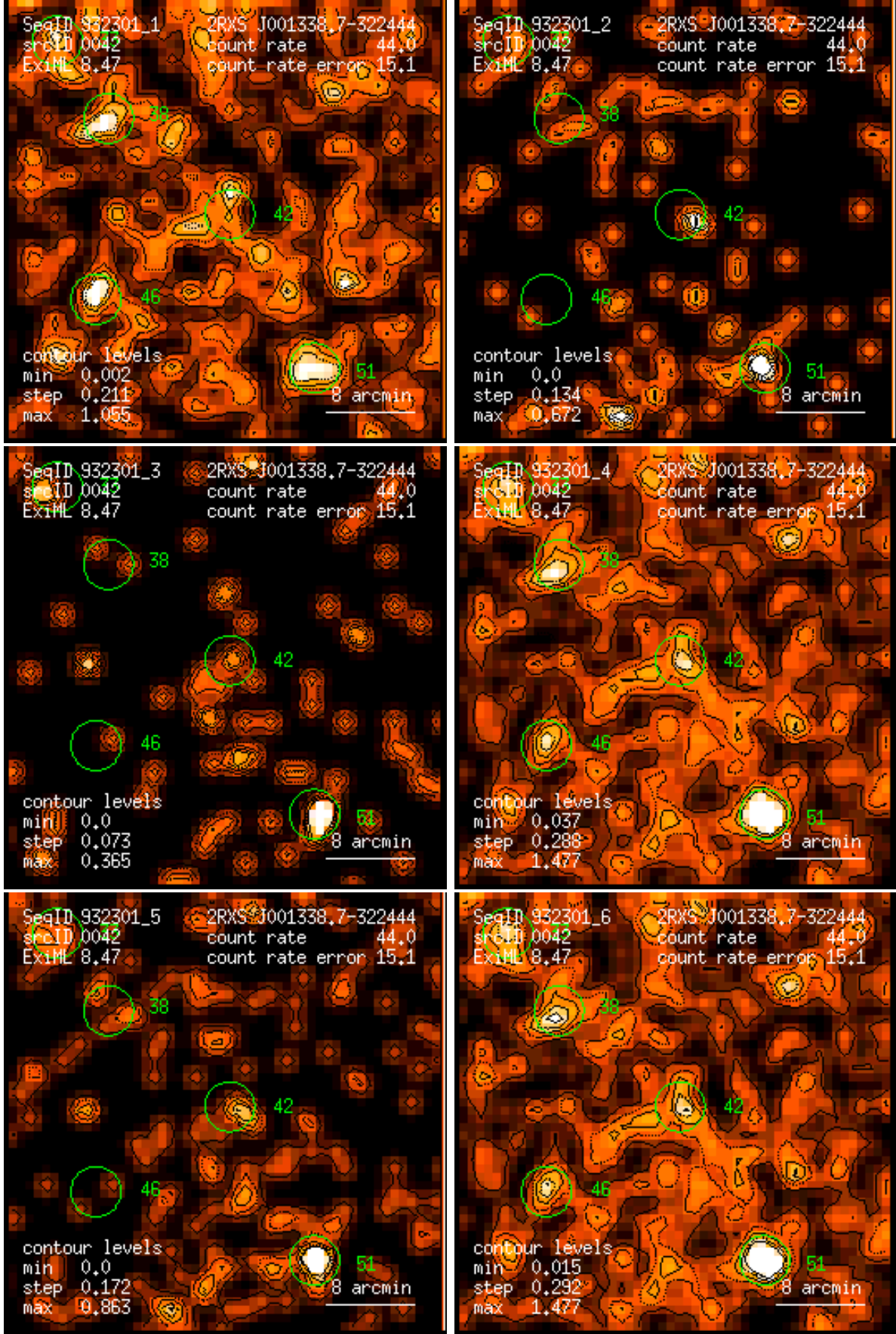
Figure 42: RASS 932301: detection 0042: band rate images, Gaussian filter: (1) PSPC channels 11 – 41, (2) 52 – 90, (3) 91 – 201, (4) 11 – 235, (5) 52 – 201, (6) 11 – 201. Broad band rates in counts/ks. Band rate contour levels in counts/ks/arcmin 2 .
