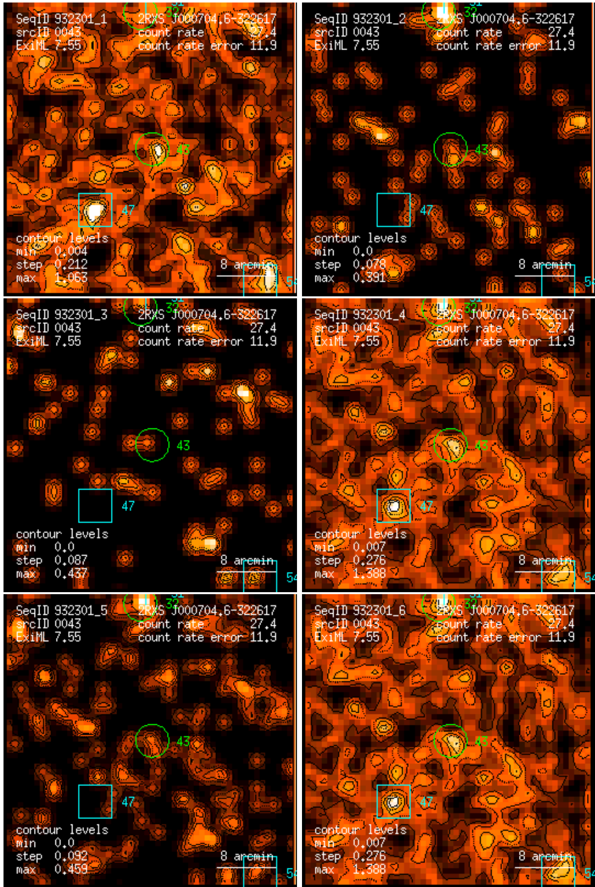
Figure 43: RASS 932301: detection 0043: band rate images, Gaussian filter: (1) PSPC channels 11 – 41, (2) 52 – 90, (3) 91 – 201, (4) 11 – 235, (5) 52 – 201, (6) 11 – 201. Broad band rates in counts/ks. Band rate contour levels in counts/ks/arcmin 2 .
