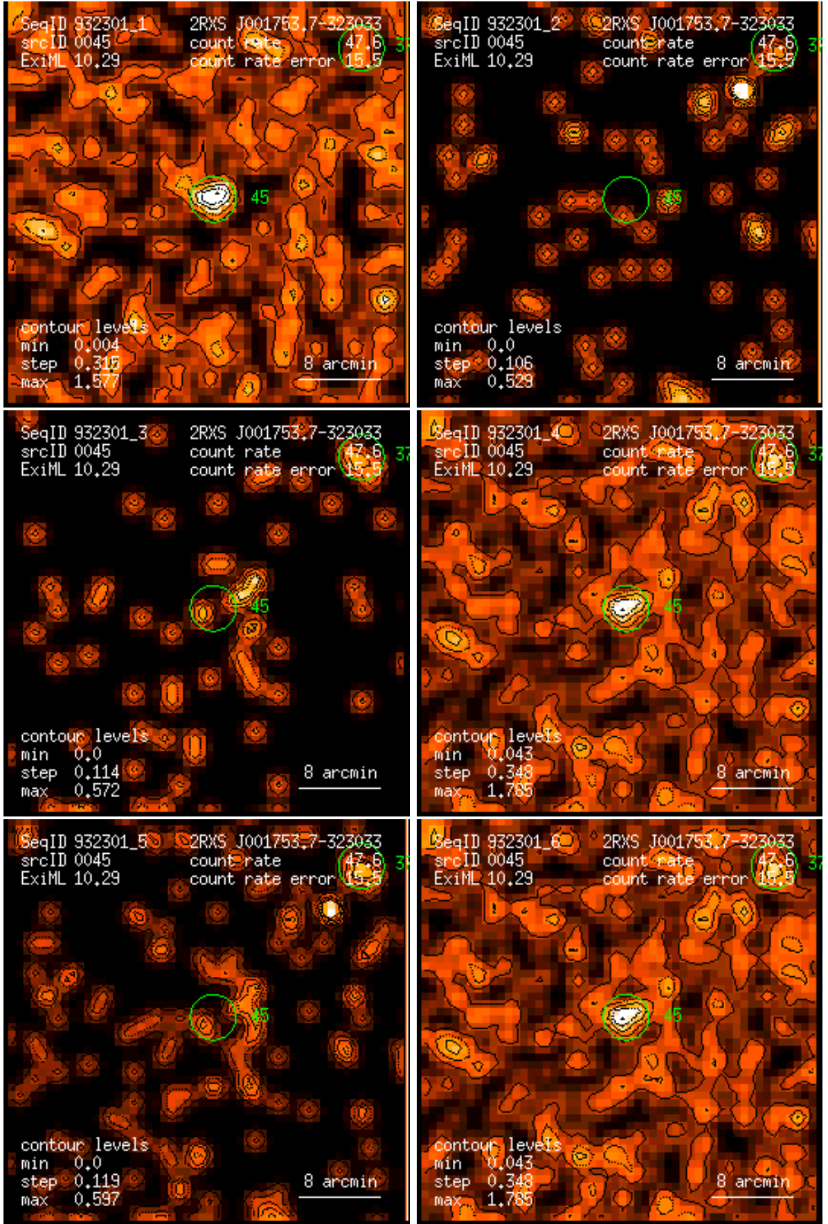
Figure 45: RASS 932301: detection 0045: band rate images, Gaussian filter: (1) PSPC channels 11 – 41, (2) 52 – 90, (3) 91 – 201, (4) 11 – 235, (5) 52 – 201, (6) 11 – 201. Broad band rates in counts/ks. Band rate contour levels in counts/ks/arcmin 2 .
