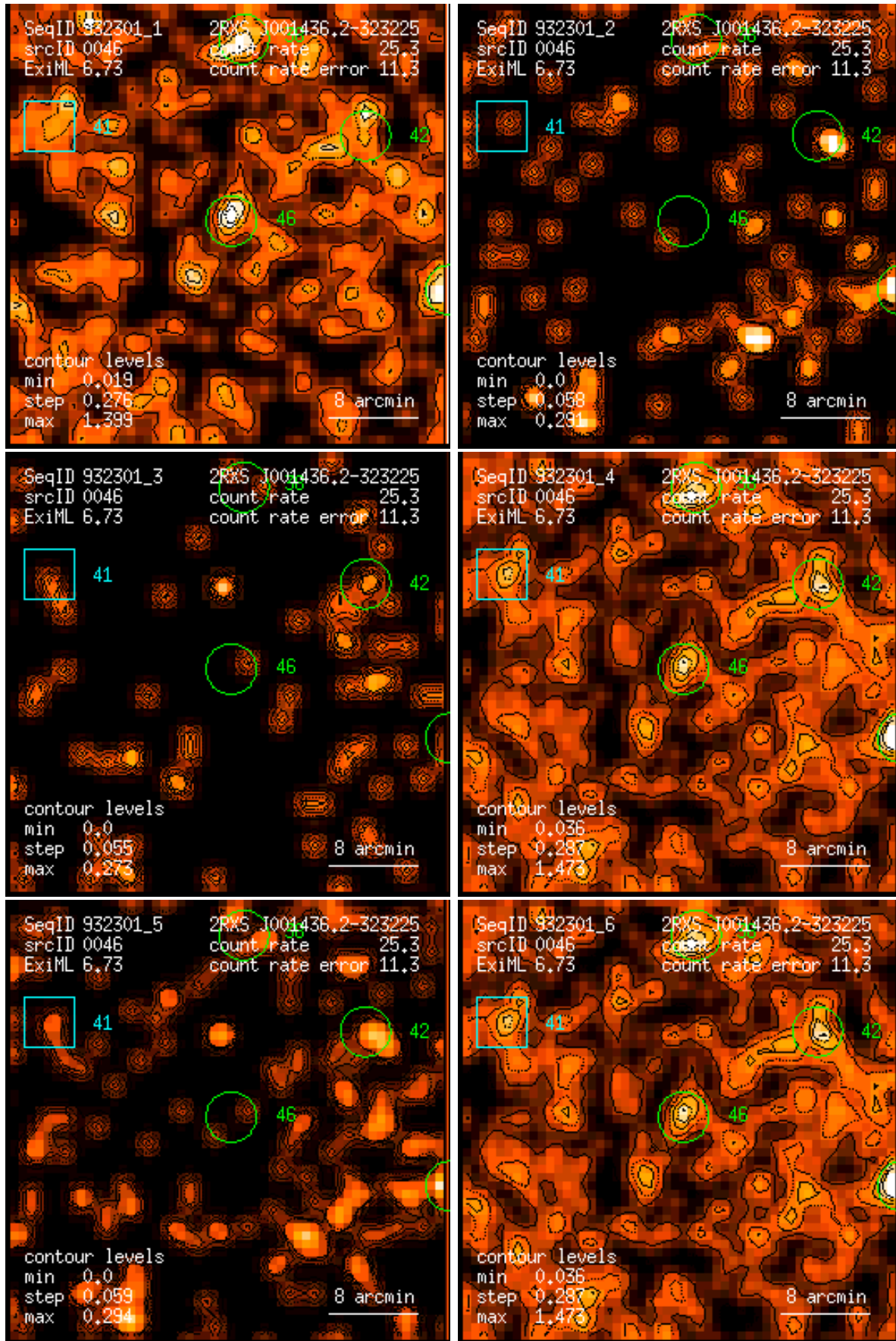
Figure 46: RASS 932301: detection 0046: band rate images, Gaussian filter: (1) PSPC channels 11 – 41, (2) 52 – 90, (3) 91 – 201, (4) 11 – 235, (5) 52 – 201, (6) 11 – 201. Broad band rates in counts/ks. Band rate contour levels in counts/ks/arcmin 2 .
