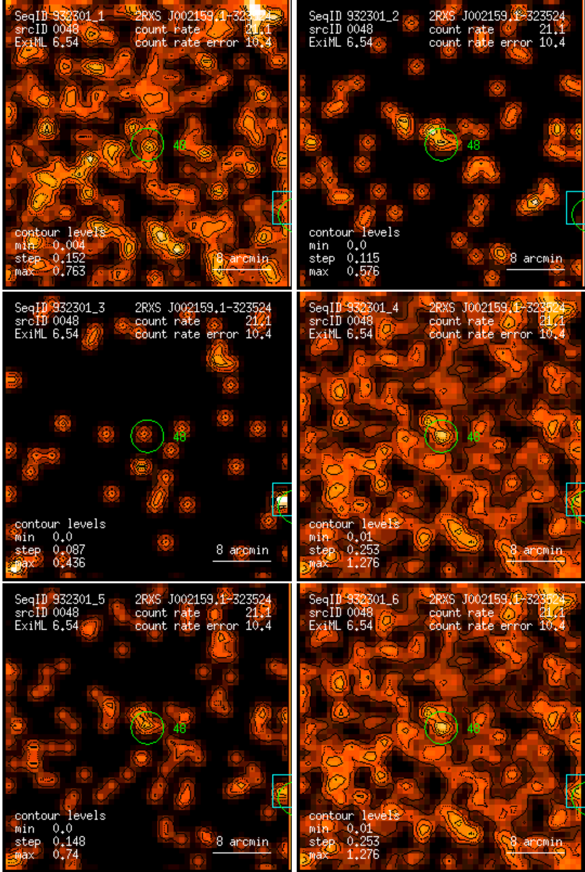
Figure 48: RASS 932301: detection 0048: band rate images, Gaussian filter: (1) PSPC channels 11 – 41, (2) 52 – 90, (3) 91 – 201, (4) 11 – 235, (5) 52 – 201, (6) 11 – 201. Broad band rates in counts/ks. Band rate contour levels in counts/ks/arcmin 2 .
