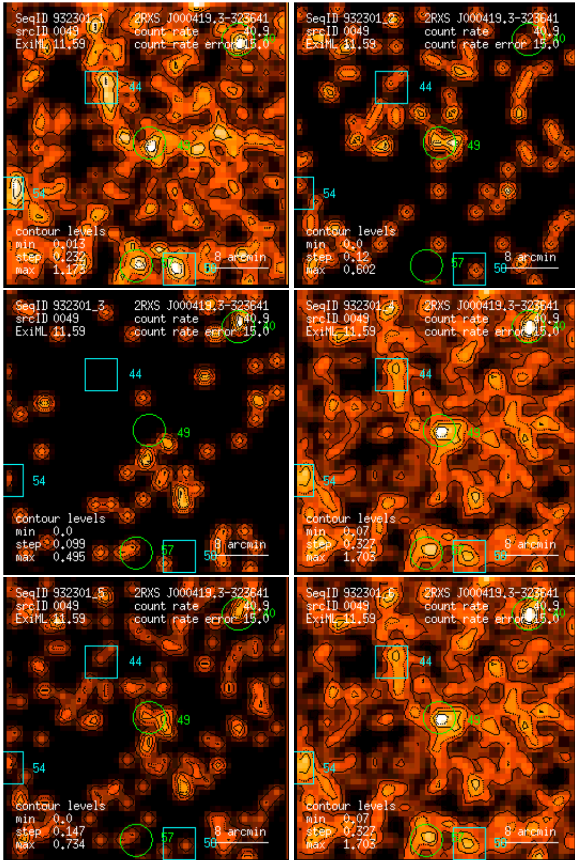
Figure 49: RASS 932301: detection 0049: band rate images, Gaussian filter: (1) PSPC channels 11 – 41, (2) 52 – 90, (3) 91 – 201, (4) 11 – 235, (5) 52 – 201, (6) 11 – 201. Broad band rates in counts/ks. Band rate contour levels in counts/ks/arcmin 2 .
