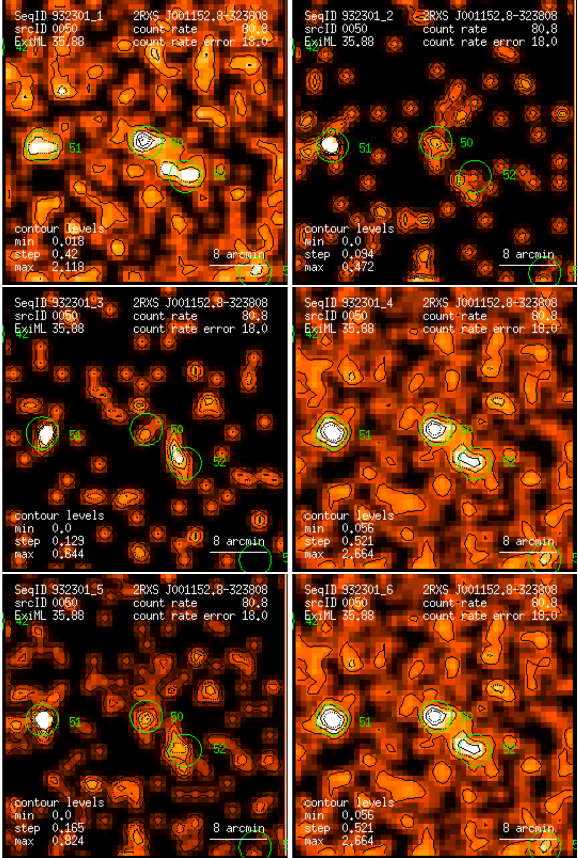
Figure 50: RASS 932301: detection 0050: band rate images, Gaussian filter: (1) PSPC channels 11 – 41, (2) 52 – 90, (3) 91 – 201, (4) 11 – 235, (5) 52 – 201, (6) 11 – 201. Broad band rates in counts/ks. Band rate contour levels in counts/ks/arcmin 2 .
