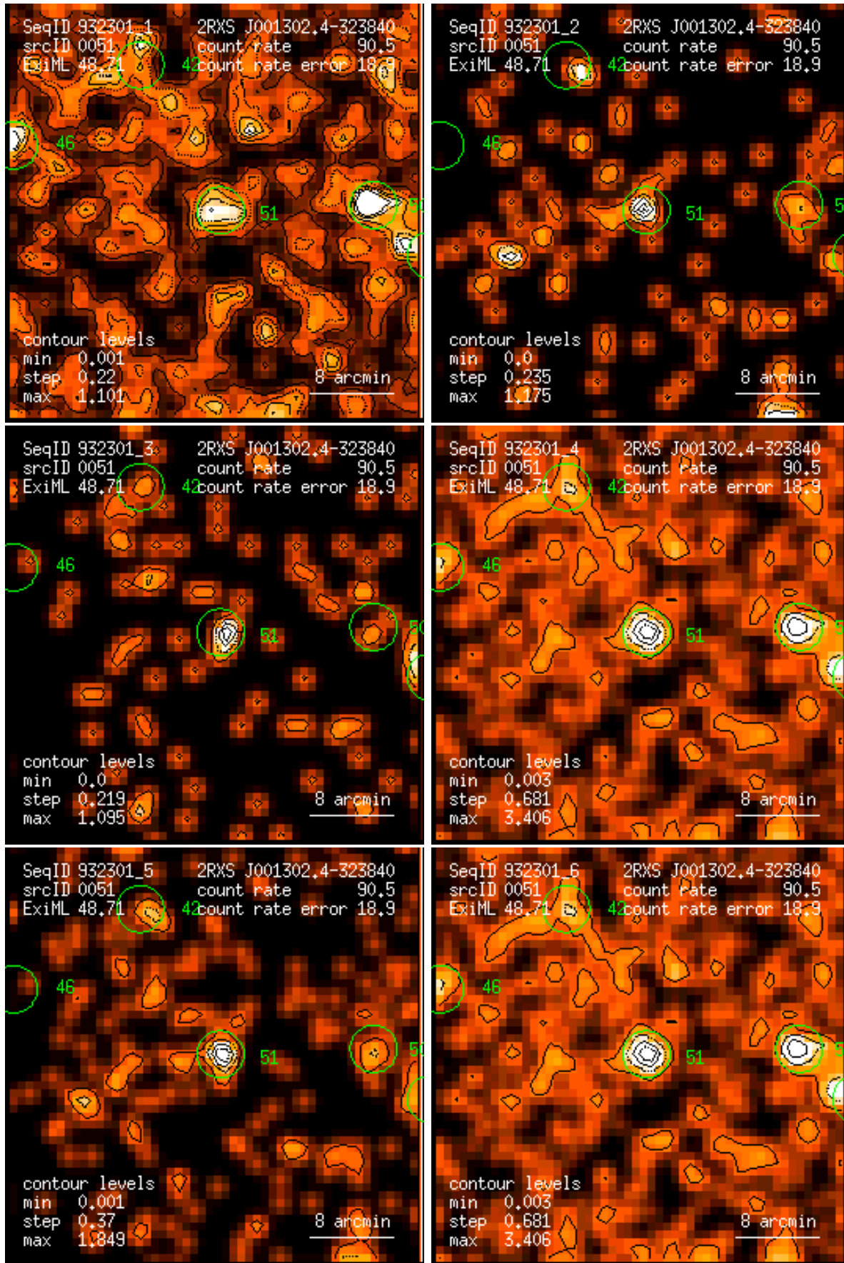
Figure 51: RASS 932301: detection 0051: band rate images, Gaussian filter: (1) PSPC channels 11 – 41, (2) 52 – 90, (3) 91 – 201, (4) 11 – 235, (5) 52 – 201, (6) 11 – 201. Broad band rates in counts/ks. Band rate contour levels in counts/ks/arcmin 2 .
