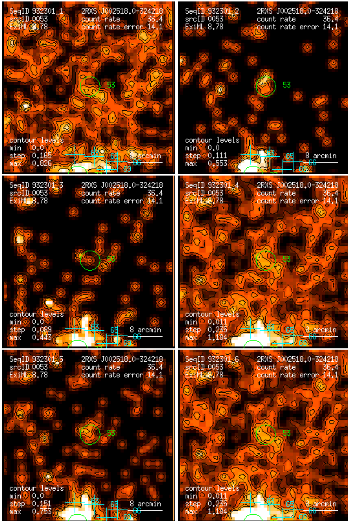
Figure 53: RASS 932301: detection 0053: band rate images, Gaussian filter: (1) PSPC channels 11 – 41, (2) 52 – 90, (3) 91 – 201, (4) 11 – 235, (5) 52 – 201, (6) 11 – 201. Broad band rates in counts/ks. Band rate contour levels in counts/ks/arcmin 2 .
