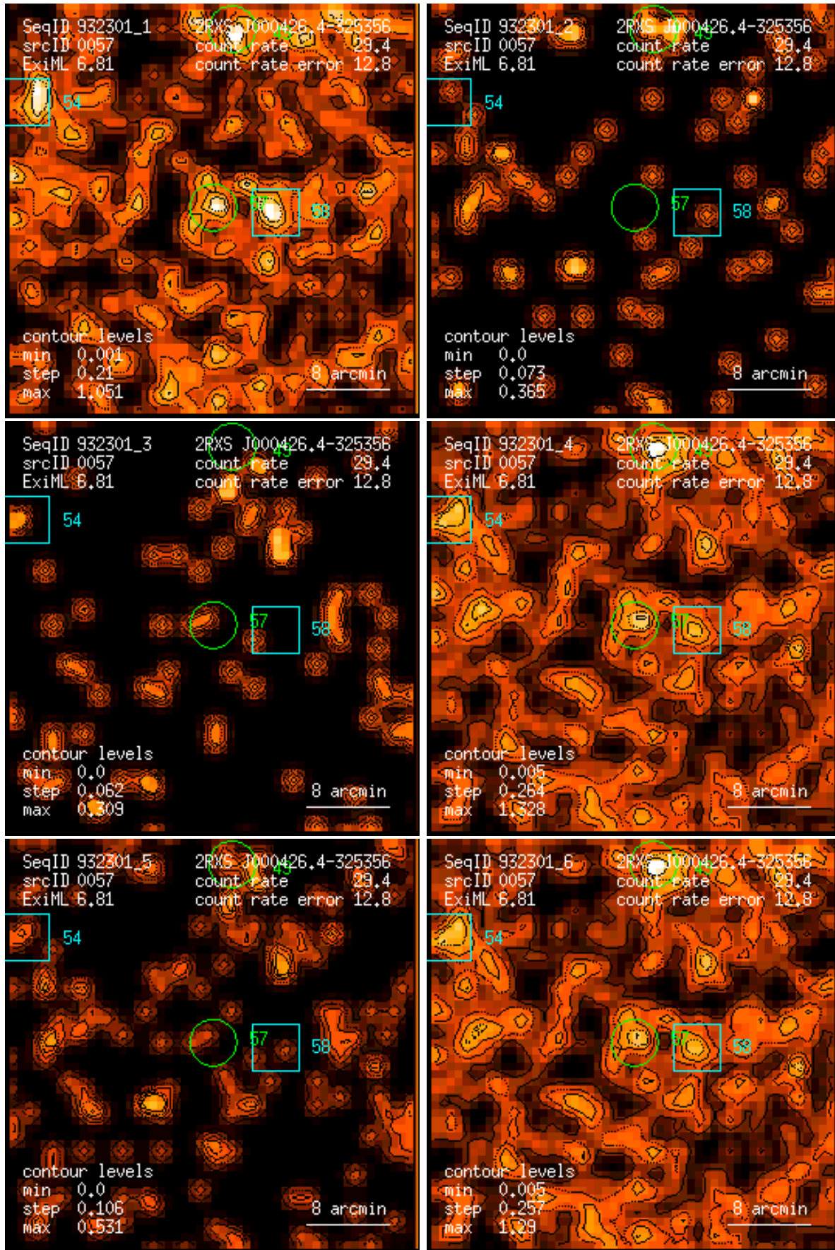
Figure 57: RASS 932301: detection 0057: band rate images, Gaussian filter: (1) PSPC channels 11 – 41, (2) 52 – 90, (3) 91 – 201, (4) 11 – 235, (5) 52 – 201, (6) 11 – 201. Broad band rates in counts/ks. Band rate contour levels in counts/ks/arcmin 2 .
