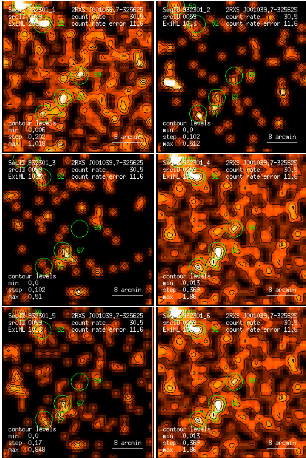
Figure 59: RASS 932301: detection 0059: band rate images, Gaussian filter: (1) PSPC channels 11 – 41, (2) 52 – 90, (3) 91 – 201, (4) 11 – 235, (5) 52 – 201, (6) 11 – 201. Broad band rates in counts/ks. Band rate contour levels in counts/ks/arcmin 2 .
