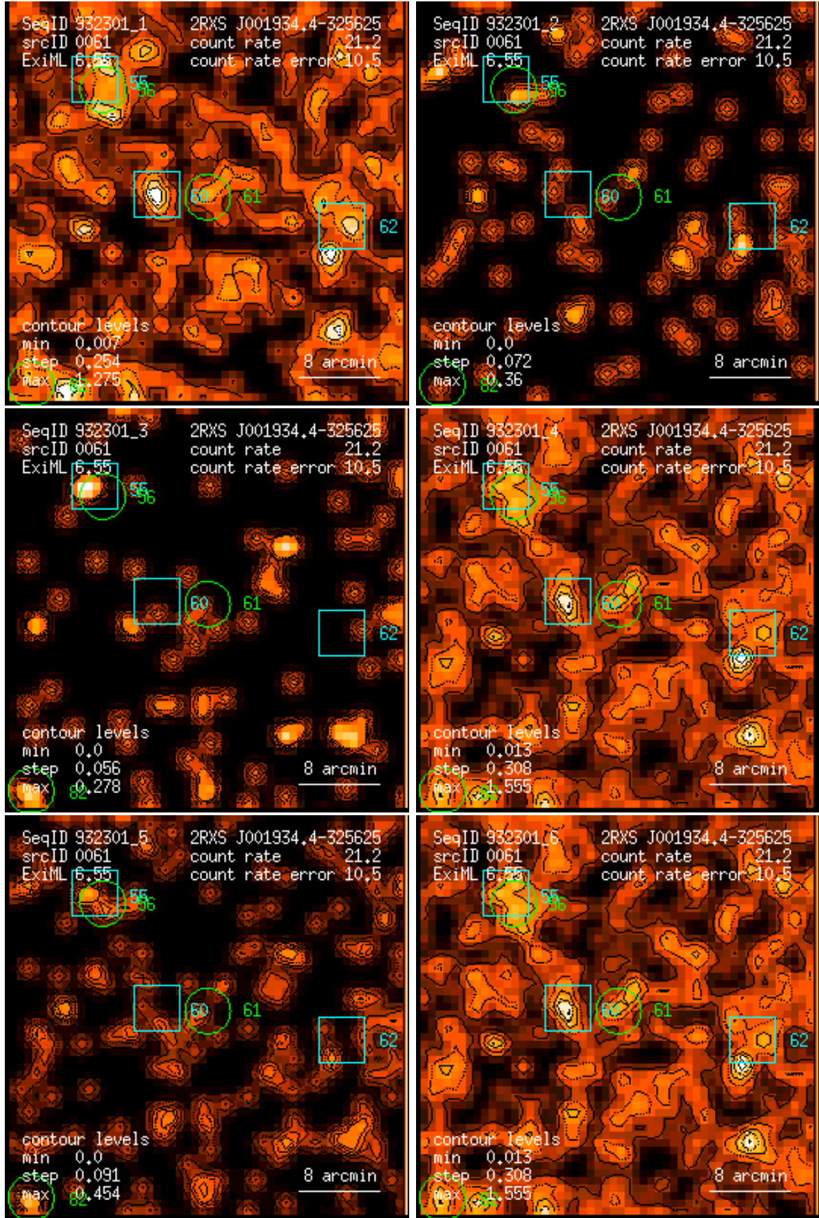
Figure 61: RASS 932301: detection 0061: band rate images, Gaussian filter: (1) PSPC channels 11 – 41, (2) 52 – 90, (3) 91 – 201, (4) 11 – 235, (5) 52 – 201, (6) 11 – 201. Broad band rates in counts/ks. Band rate contour levels in counts/ks/arcmin 2 .
