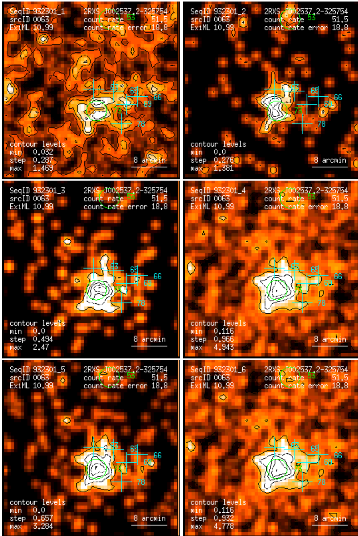
Figure 63: RASS 932301: detection 0063: band rate images, Gaussian filter: (1) PSPC channels 11 – 41, (2) 52 – 90, (3) 91 – 201, (4) 11 – 235, (5) 52 – 201, (6) 11 – 201. Broad band rates in counts/ks. Band rate contour levels in counts/ks/arcmin 2 .
