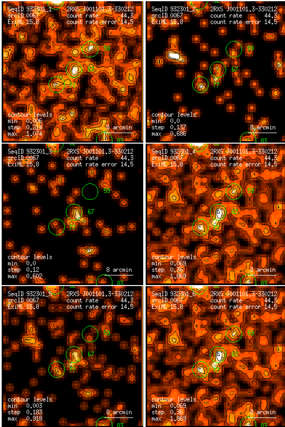
Figure 67: RASS 932301: detection 0067: band rate images, Gaussian filter: (1) PSPC channels 11 – 41, (2) 52 – 90, (3) 91 – 201, (4) 11 – 235, (5) 52 – 201, (6) 11 – 201. Broad band rates in counts/ks. Band rate contour levels in counts/ks/arcmin 2 .
