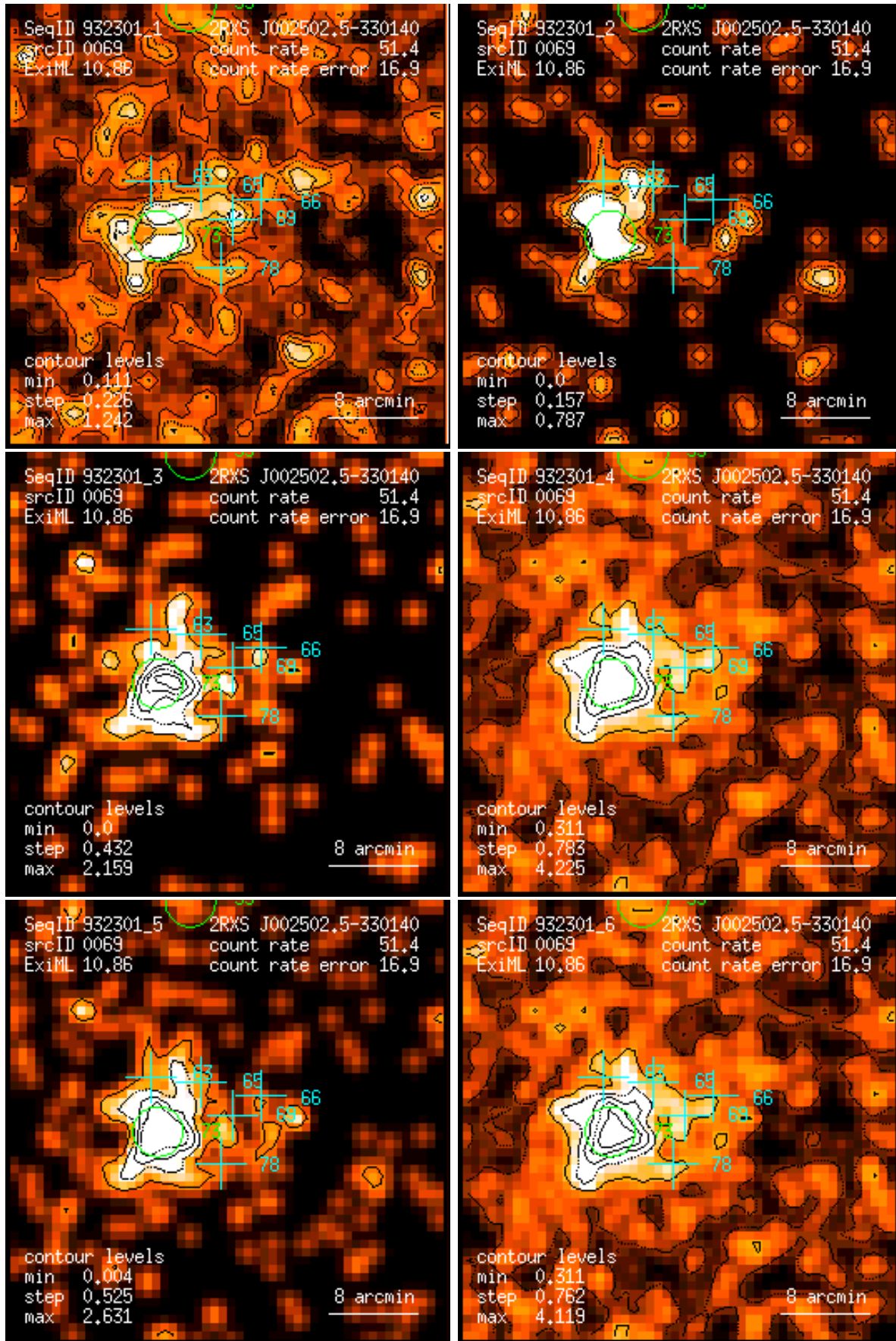
Figure 69: RASS 932301: detection 0069: band rate images, Gaussian filter: (1) PSPC channels 11 – 41, (2) 52 – 90, (3) 91 – 201, (4) 11 – 235, (5) 52 – 201, (6) 11 – 201. Broad band rates in counts/ks. Band rate contour levels in counts/ks/arcmin 2 .
