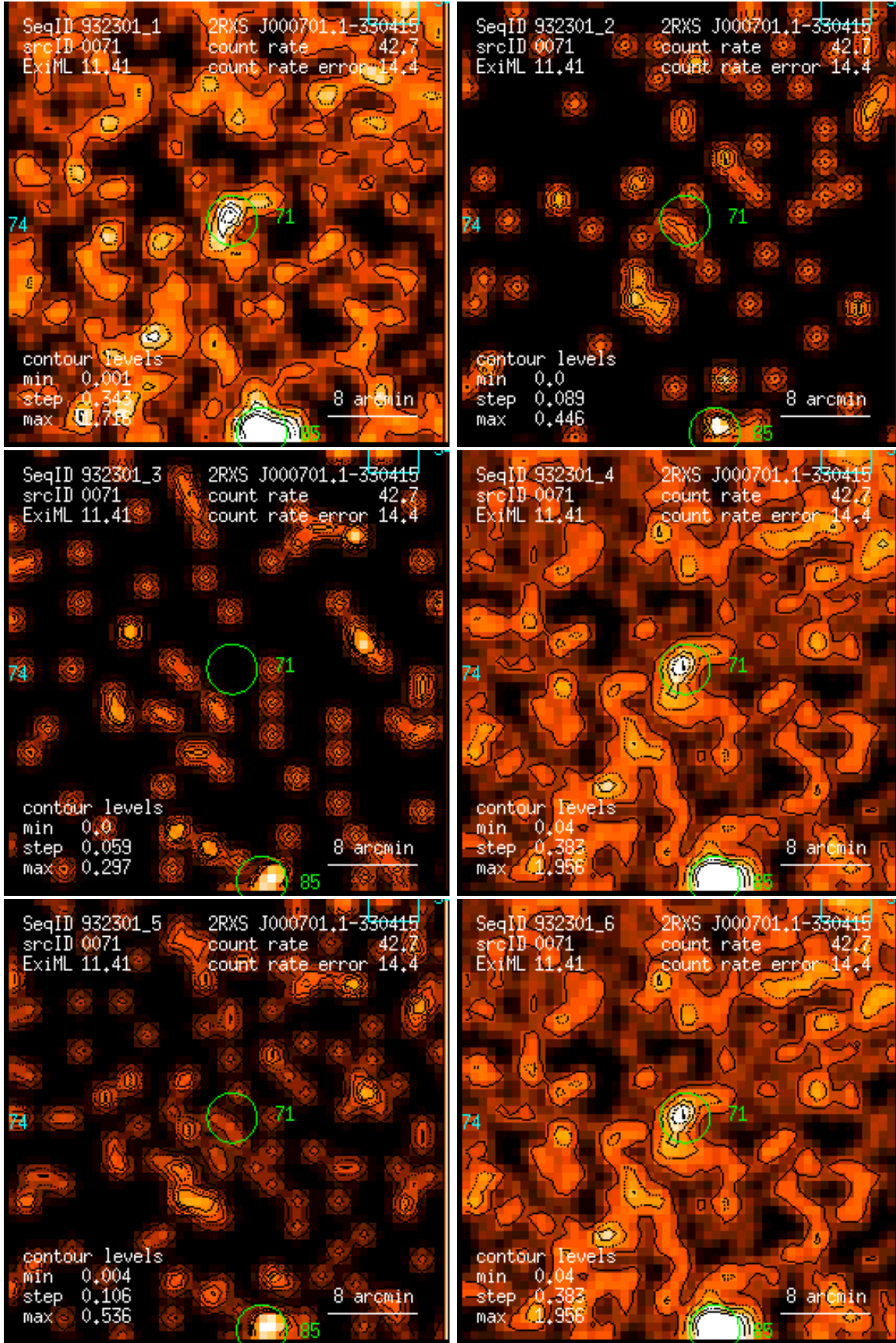
Figure 71: RASS 932301: detection 0071: band rate images, Gaussian filter: (1) PSPC channels 11 – 41, (2) 52 – 90, (3) 91 – 201, (4) 11 – 235, (5) 52 – 201, (6) 11 – 201. Broad band rates in counts/ks. Band rate contour levels in counts/ks/arcmin 2 .
