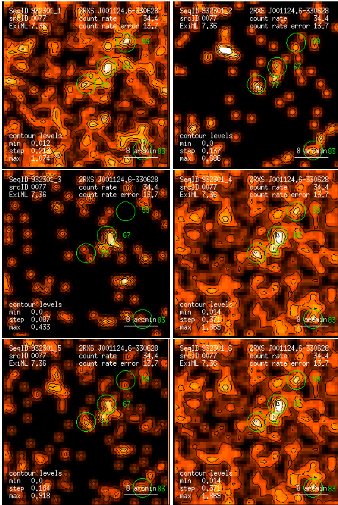
Figure 77: RASS 932301: detection 0077: band rate images, Gaussian filter: (1) PSPC channels 11 – 41, (2) 52 – 90, (3) 91 – 201, (4) 11 – 235, (5) 52 – 201, (6) 11 – 201. Broad band rates in counts/ks. Band rate contour levels in counts/ks/arcmin 2 .
