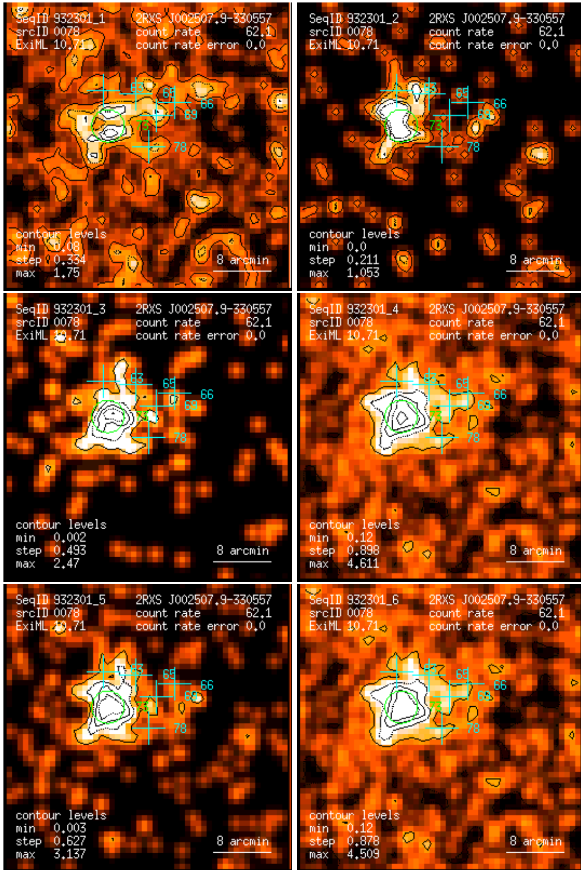
Figure 78: RASS 932301: detection 0078: band rate images, Gaussian filter: (1) PSPC channels 11 – 41, (2) 52 – 90, (3) 91 – 201, (4) 11 – 235, (5) 52 – 201, (6) 11 – 201. Broad band rates in counts/ks. Band rate contour levels in counts/ks/arcmin 2 .
