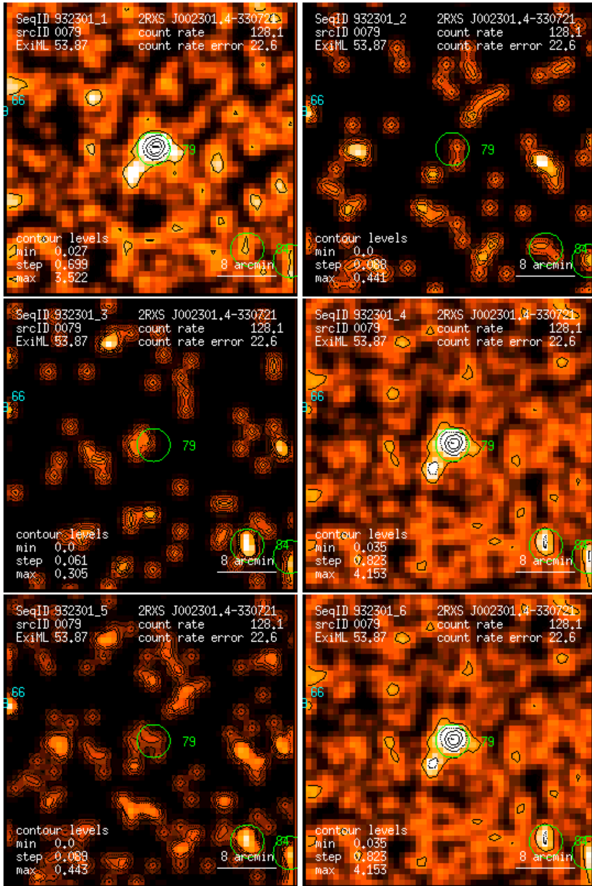
Figure 79: RASS 932301: detection 0079: band rate images, Gaussian filter: (1) PSPC channels 11 – 41, (2) 52 – 90, (3) 91 – 201, (4) 11 – 235, (5) 52 – 201, (6) 11 – 201. Broad band rates in counts/ks. Band rate contour levels in counts/ks/arcmin 2 .
