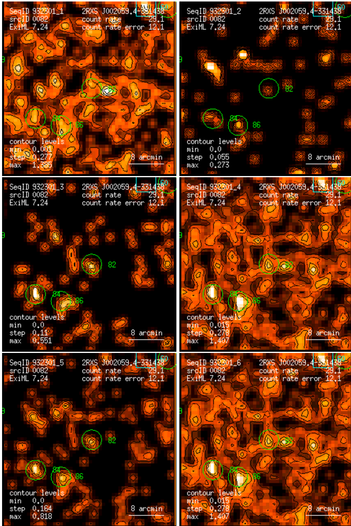
Figure 82: RASS 932301: detection 0082: band rate images, Gaussian filter: (1) PSPC channels 11 – 41, (2) 52 – 90, (3) 91 – 201, (4) 11 – 235, (5) 52 – 201, (6) 11 – 201. Broad band rates in counts/ks. Band rate contour levels in counts/ks/arcmin 2 .
