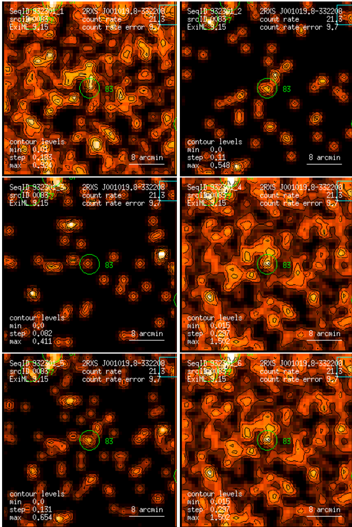
Figure 83: RASS 932301: detection 0083: band rate images, Gaussian filter: (1) PSPC channels 11 – 41, (2) 52 – 90, (3) 91 – 201, (4) 11 – 235, (5) 52 – 201, (6) 11 – 201. Broad band rates in counts/ks. Band rate contour levels in counts/ks/arcmin 2 .
