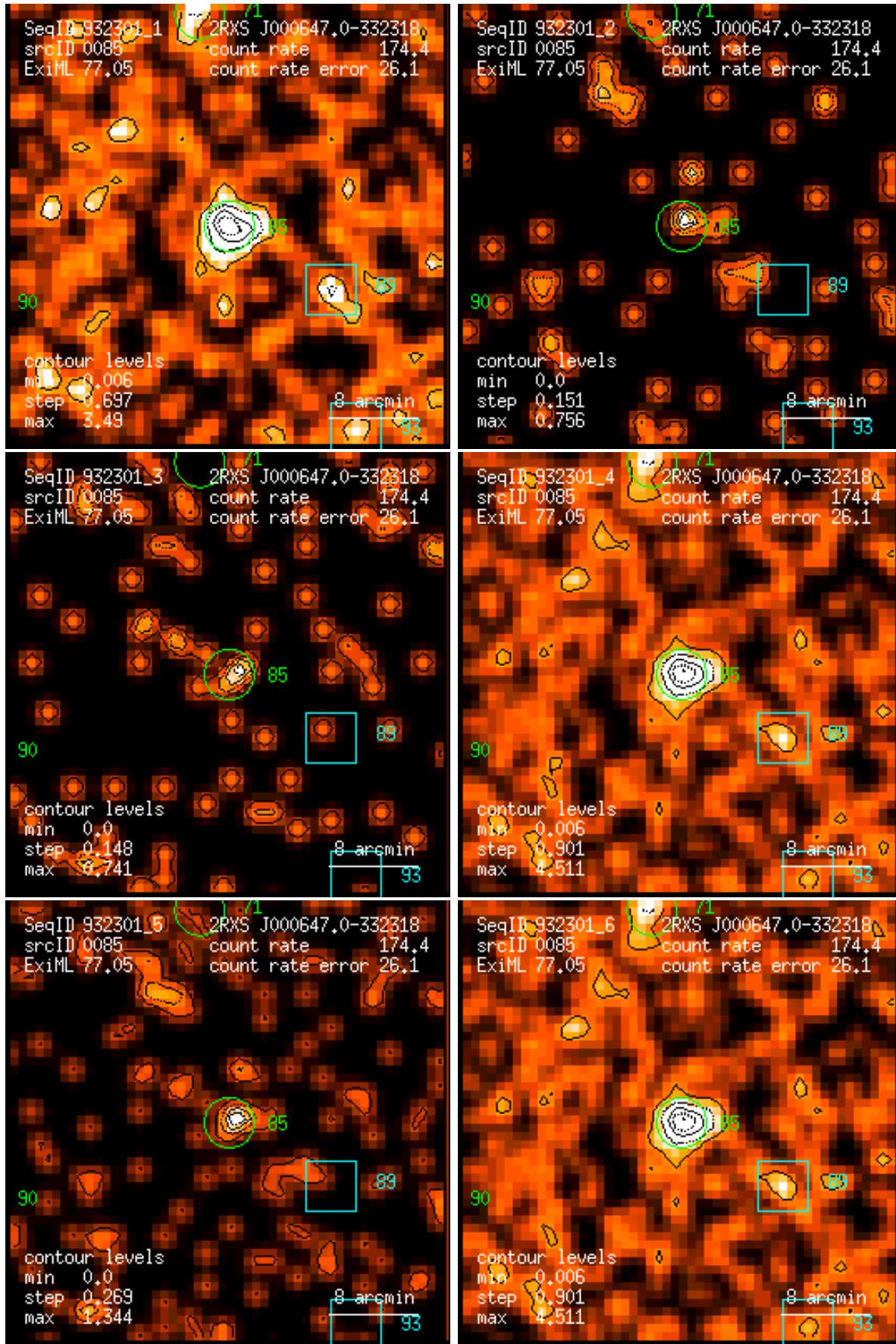
Figure 85: RASS 932301: detection 0085: band rate images, Gaussian filter: (1) PSPC channels 11 – 41, (2) 52 – 90, (3) 91 – 201, (4) 11 – 235, (5) 52 – 201, (6) 11 – 201. Broad band rates in counts/ks. Band rate contour levels in counts/ks/arcmin 2 .
