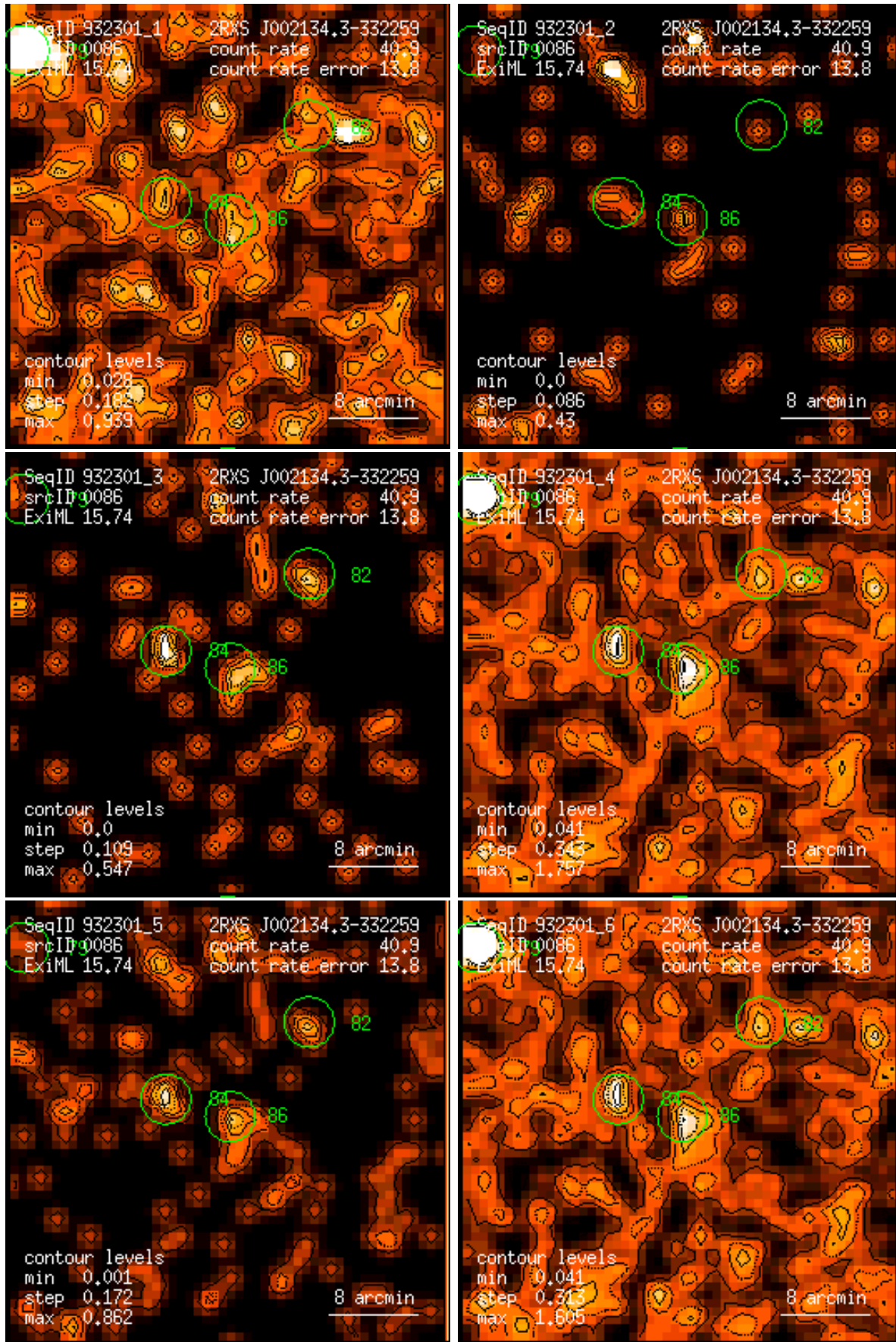
Figure 86: RASS 932301: detection 0086: band rate images, Gaussian filter: (1) PSPC channels 11 – 41, (2) 52 – 90, (3) 91 – 201, (4) 11 – 235, (5) 52 – 201, (6) 11 – 201. Broad band rates in counts/ks. Band rate contour levels in counts/ks/arcmin 2 .
