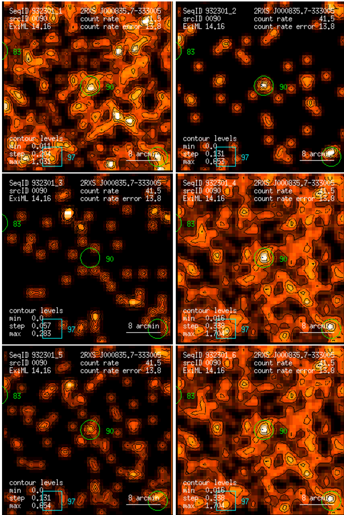
Figure 90: RASS 932301: detection 0090: band rate images, Gaussian filter: (1) PSPC channels 11 – 41, (2) 52 – 90, (3) 91 – 201, (4) 11 – 235, (5) 52 – 201, (6) 11 – 201. Broad band rates in counts/ks. Band rate contour levels in counts/ks/arcmin 2 .
