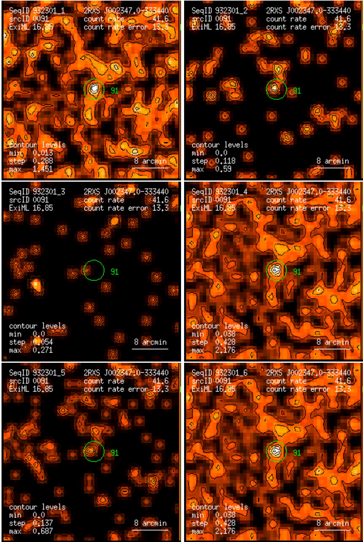
Figure 91: RASS 932301: detection 0091: band rate images, Gaussian filter: (1) PSPC channels 11 – 41, (2) 52 – 90, (3) 91 – 201, (4) 11 – 235, (5) 52 – 201, (6) 11 – 201. Broad band rates in counts/ks. Band rate contour levels in counts/ks/arcmin 2 .
