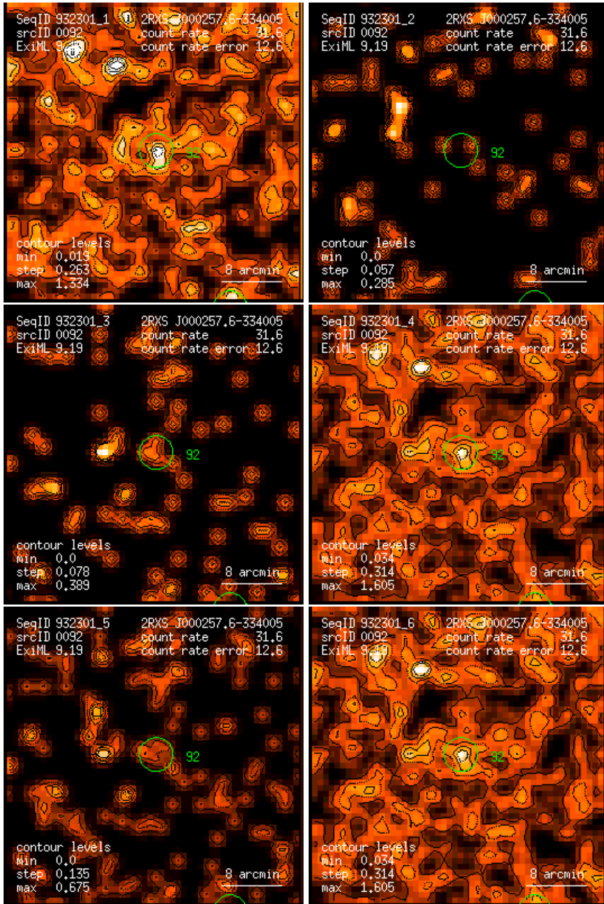
Figure 92: RASS 932301: detection 0092: band rate images, Gaussian filter: (1) PSPC channels 11 – 41, (2) 52 – 90, (3) 91 – 201, (4) 11 – 235, (5) 52 – 201, (6) 11 – 201. Broad band rates in counts/ks. Band rate contour levels in counts/ks/arcmin 2 .
