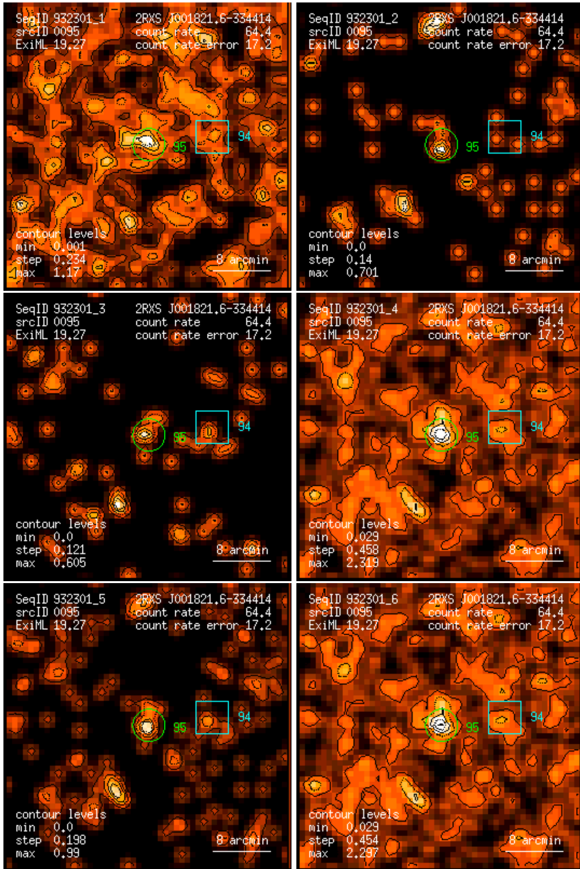
Figure 95: RASS 932301: detection 0095: band rate images, Gaussian filter: (1) PSPC channels 11 – 41, (2) 52 – 90, (3) 91 – 201, (4) 11 – 235, (5) 52 – 201, (6) 11 – 201. Broad band rates in counts/ks. Band rate contour levels in counts/ks/arcmin 2 .
