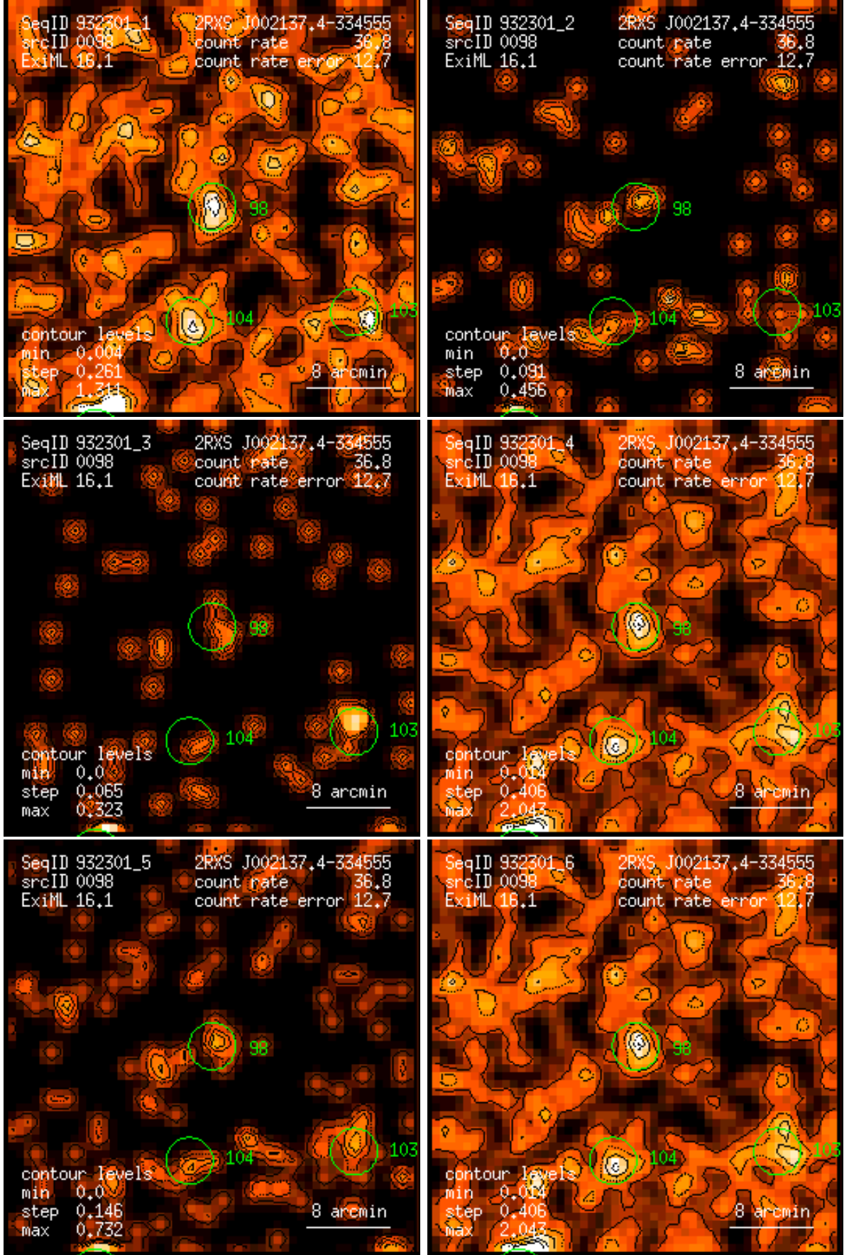
Figure 98: RASS 932301: detection 0098: band rate images, Gaussian filter: (1) PSPC channels 11 – 41, (2) 52 – 90, (3) 91 – 201, (4) 11 – 235, (5) 52 – 201, (6) 11 – 201. Broad band rates in counts/ks. Band rate contour levels in counts/ks/arcmin 2 .
