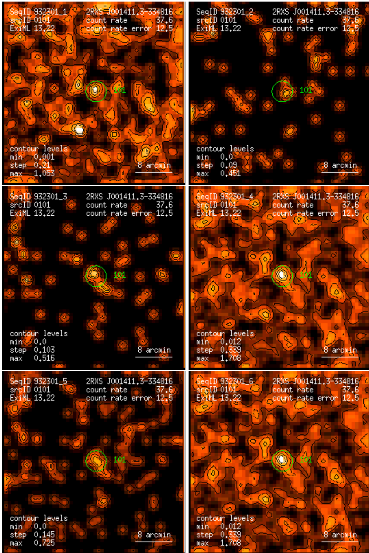
Figure 101: RASS 932301: detection 0101: band rate images, Gaussian filter: (1) PSPC channels 11 – 41, (2) 52 – 90, (3) 91 – 201, (4) 11 – 235, (5) 52 – 201, (6) 11 – 201. Broad band rates in counts/ks. Band rate contour levels in counts/ks/arcmin 2 .
