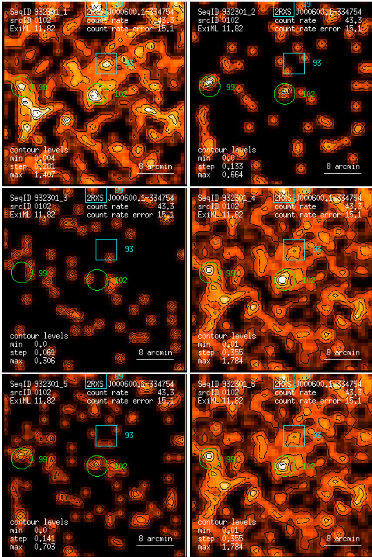
Figure 102: RASS 932301: detection 0102: band rate images, Gaussian filter: (1) PSPC channels 11 – 41, (2) 52 – 90, (3) 91 – 201, (4) 11 – 235, (5) 52 – 201, (6) 11 – 201. Broad band rates in counts/ks. Band rate contour levels in counts/ks/arcmin 2 .
