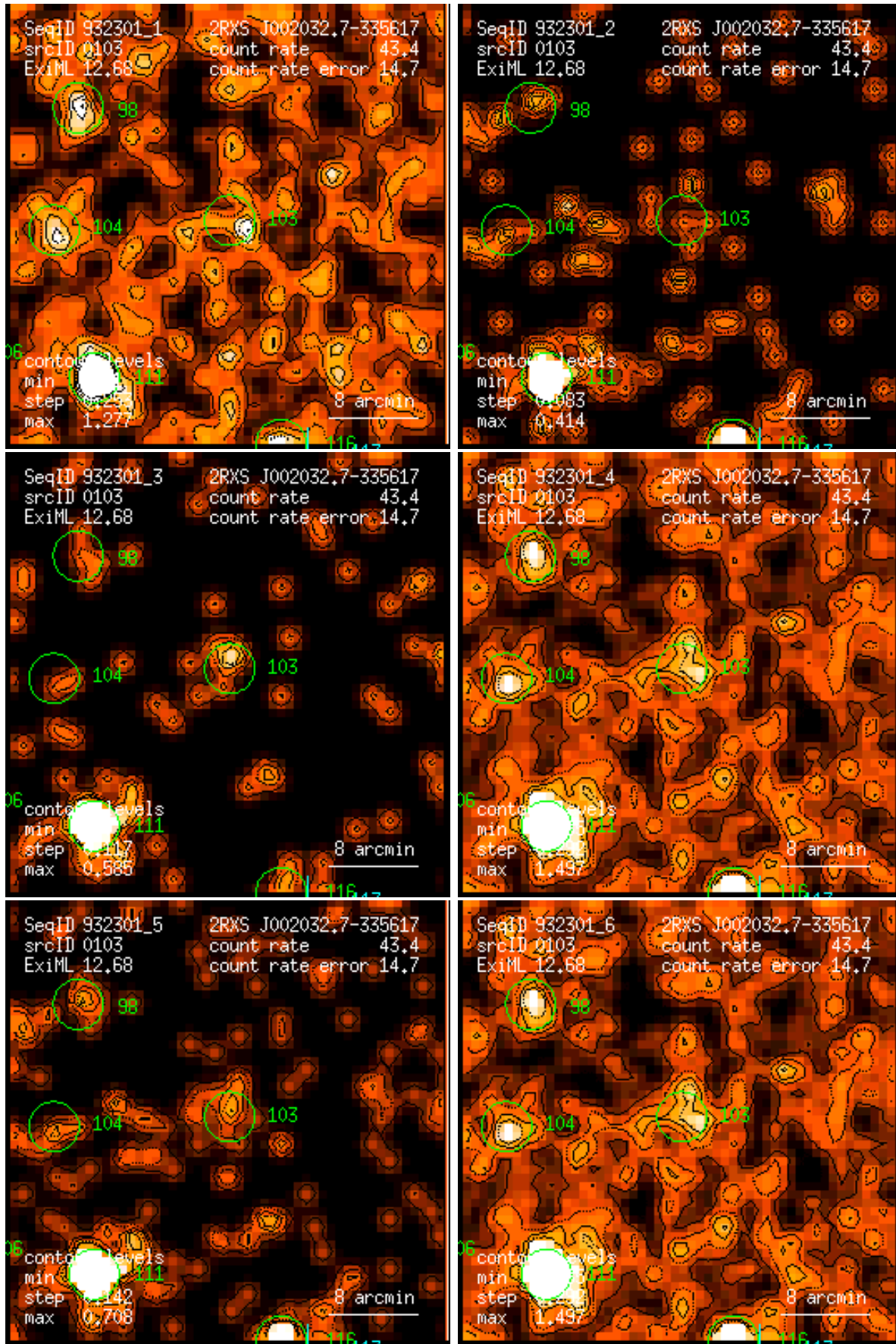
Figure 103: RASS 932301: detection 0103: band rate images, Gaussian filter: (1) PSPC channels 11 – 41, (2) 52 – 90, (3) 91 – 201, (4) 11 – 235, (5) 52 – 201, (6) 11 – 201. Broad band rates in counts/ks. Band rate contour levels in counts/ks/arcmin 2 .
