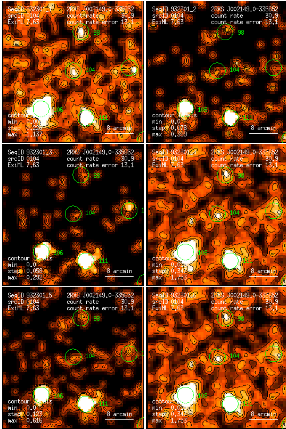
Figure 104: RASS 932301: detection 0104: band rate images, Gaussian filter: (1) PSPC channels 11 – 41, (2) 52 – 90, (3) 91 – 201, (4) 11 – 235, (5) 52 – 201, (6) 11 – 201. Broad band rates in counts/ks. Band rate contour levels in counts/ks/arcmin 2 .
