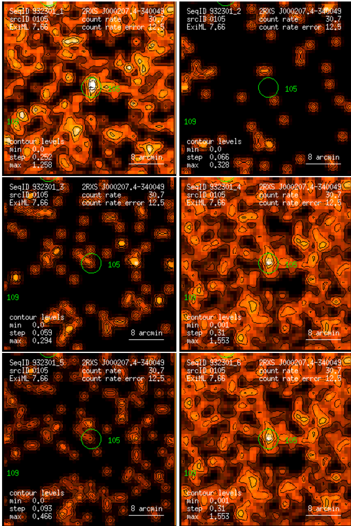
Figure 105: RASS 932301: detection 0105: band rate images, Gaussian filter: (1) PSPC channels 11 – 41, (2) 52 – 90, (3) 91 – 201, (4) 11 – 235, (5) 52 – 201, (6) 11 – 201. Broad band rates in counts/ks. Band rate contour levels in counts/ks/arcmin 2 .
