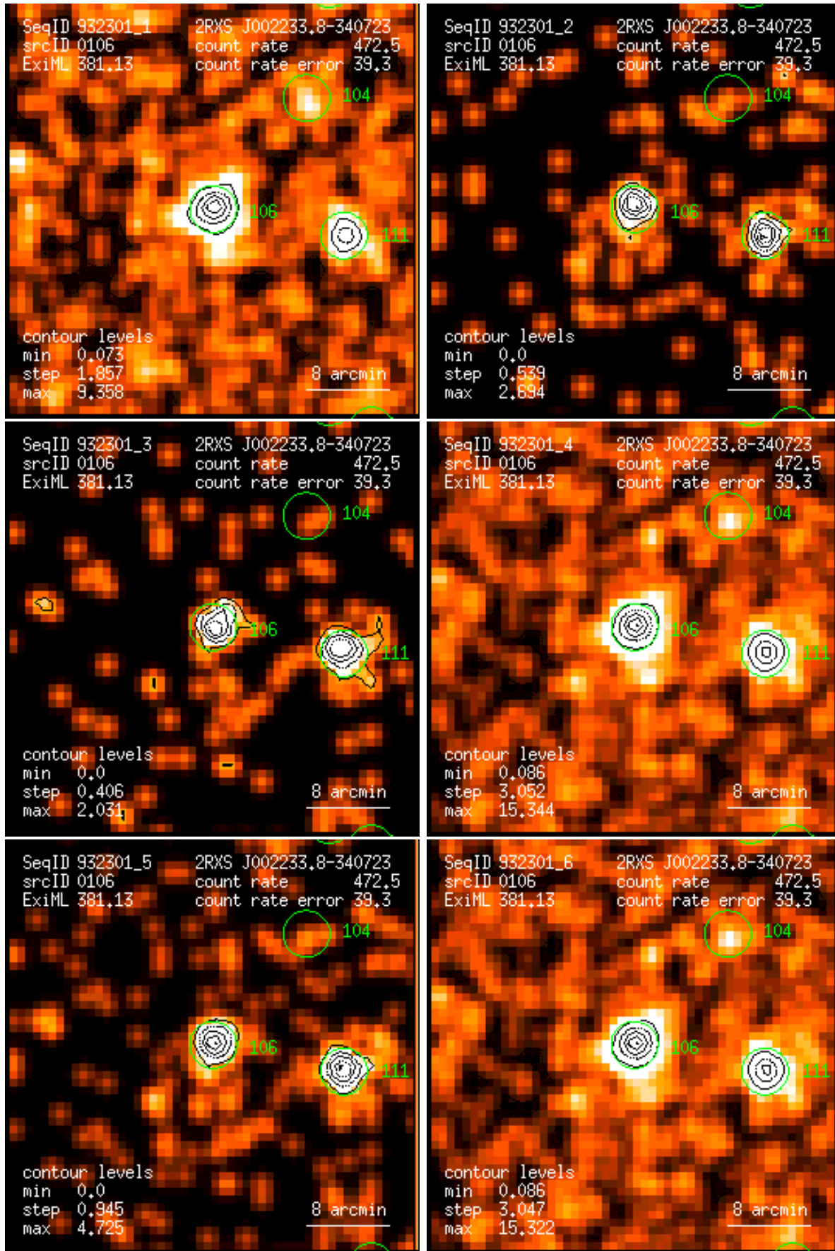
Figure 106: RASS 932301: detection 0106: band rate images, Gaussian filter: (1) PSPC channels 11 – 41, (2) 52 – 90, (3) 91 – 201, (4) 11 – 235, (5) 52 – 201, (6) 11 – 201. Broad band rates in counts/ks. Band rate contour levels in counts/ks/arcmin 2 .
