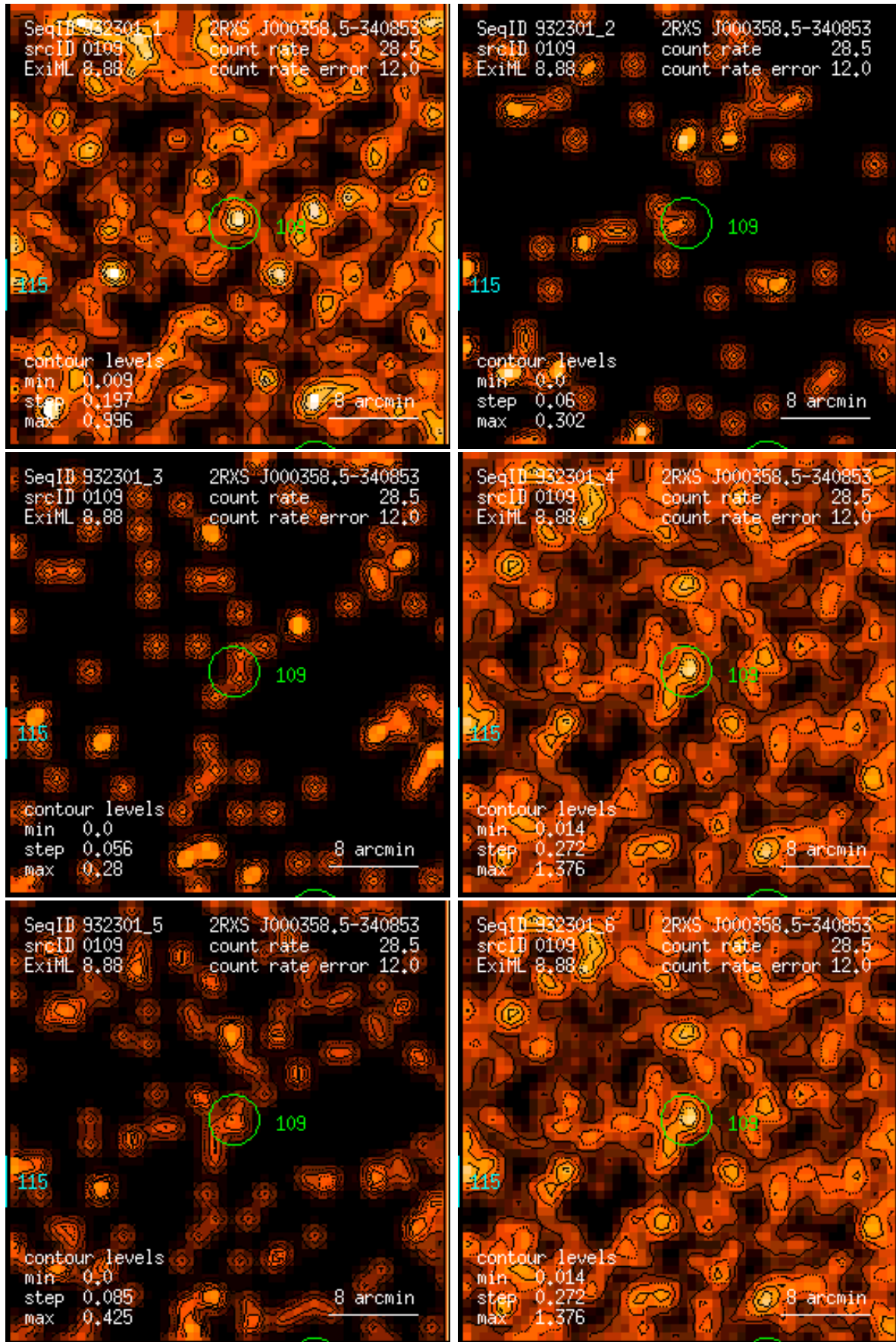
Figure 109: RASS 932301: detection 0109: band rate images, Gaussian filter: (1) PSPC channels 11 – 41, (2) 52 – 90, (3) 91 – 201, (4) 11 – 235, (5) 52 – 201, (6) 11 – 201. Broad band rates in counts/ks. Band rate contour levels in counts/ks/arcmin 2 .
