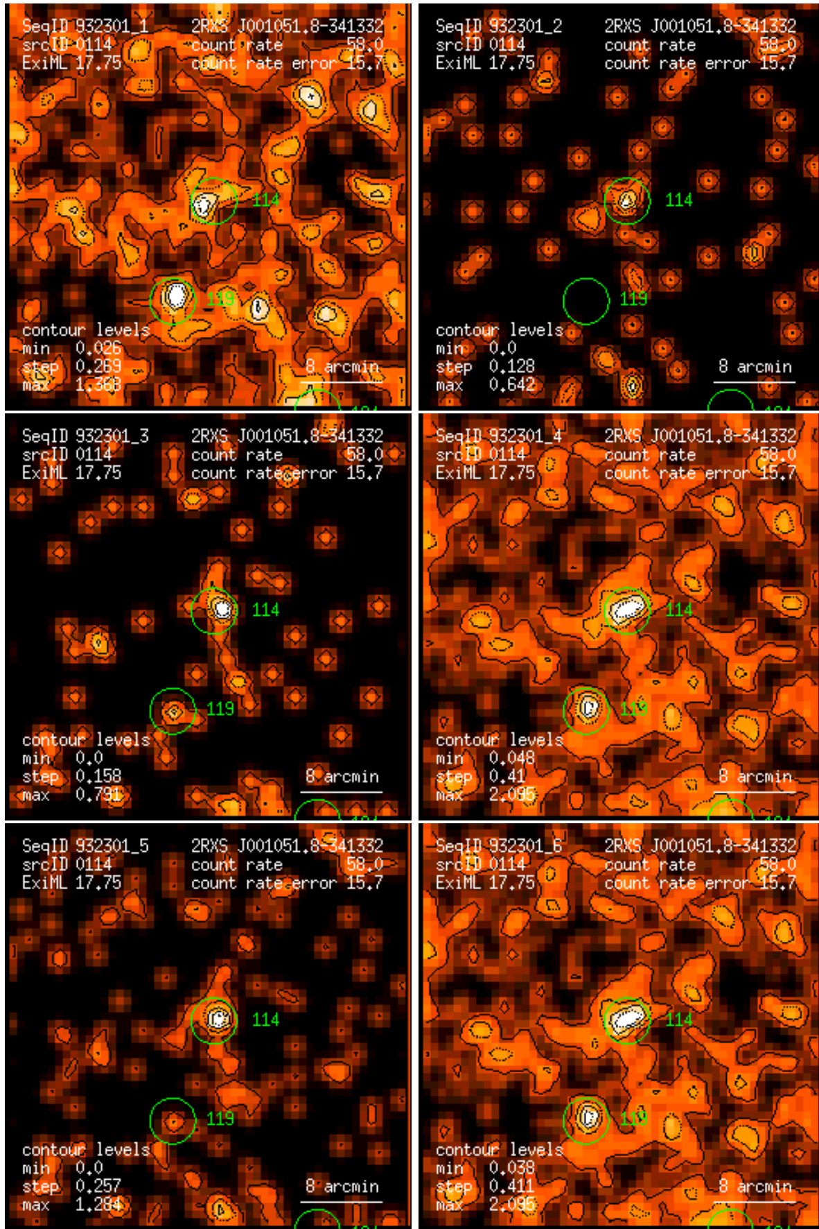
Figure 114: RASS 932301: detection 0114: band rate images, Gaussian filter: (1) PSPC channels 11 – 41, (2) 52 – 90, (3) 91 – 201, (4) 11 – 235, (5) 52 – 201, (6) 11 – 201. Broad band rates in counts/ks. Band rate contour levels in counts/ks/arcmin 2 .
