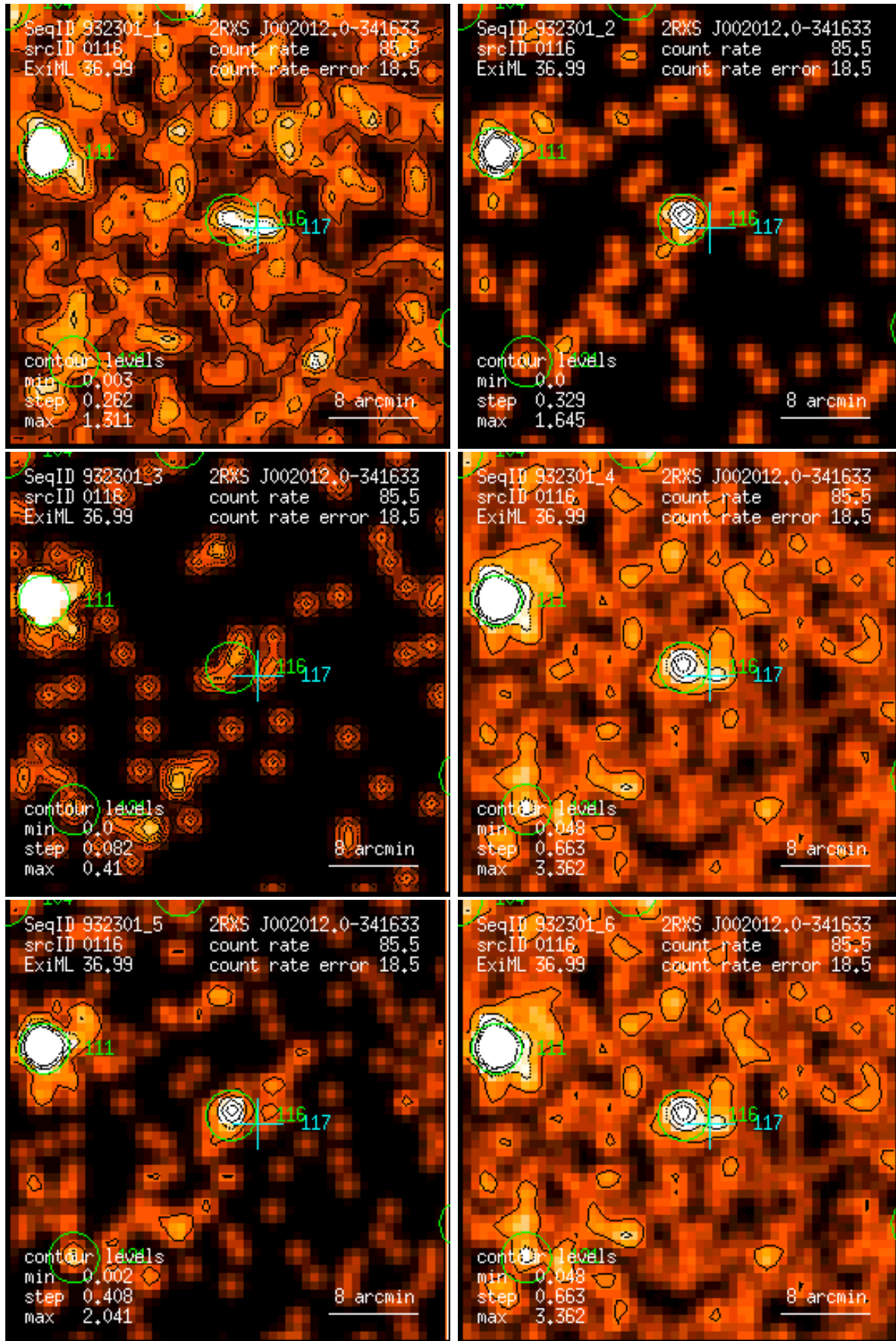
Figure 116: RASS 932301: detection 0116: band rate images, Gaussian filter: (1) PSPC channels 11 – 41, (2) 52 – 90, (3) 91 – 201, (4) 11 – 235, (5) 52 – 201, (6) 11 – 201. Broad band rates in counts/ks. Band rate contour levels in counts/ks/arcmin 2 .
