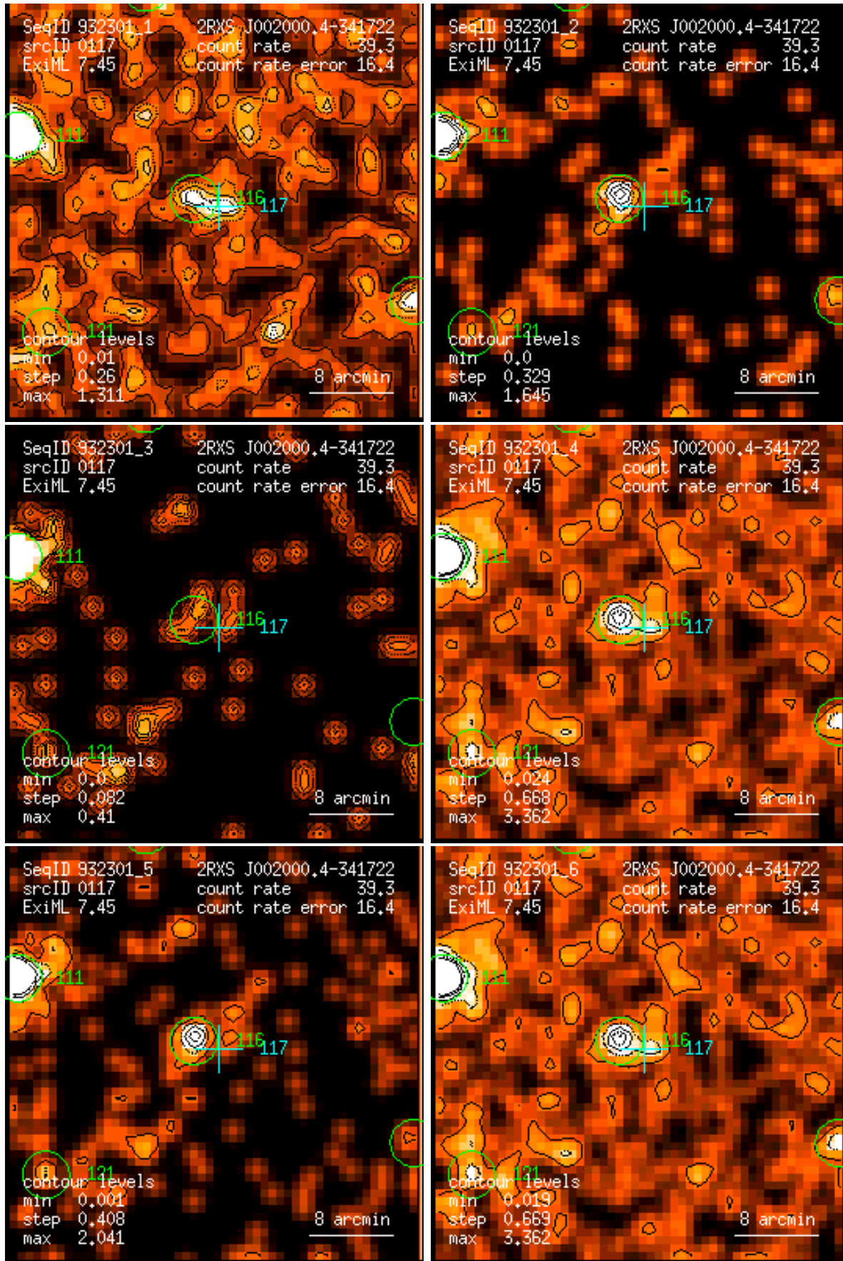
Figure 117: RASS 932301: detection 0117: band rate images, Gaussian filter: (1) PSPC channels 11 – 41, (2) 52 – 90, (3) 91 – 201, (4) 11 – 235, (5) 52 – 201, (6) 11 – 201. Broad band rates in counts/ks. Band rate contour levels in counts/ks/arcmin 2 .
