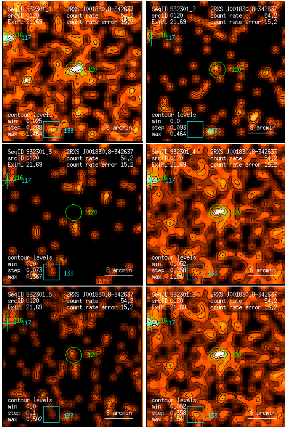
Figure 120: RASS 932301: detection 0120: band rate images, Gaussian filter: (1) PSPC channels 11 – 41, (2) 52 – 90, (3) 91 – 201, (4) 11 – 235, (5) 52 – 201, (6) 11 – 201. Broad band rates in counts/ks. Band rate contour levels in counts/ks/arcmin 2 .
