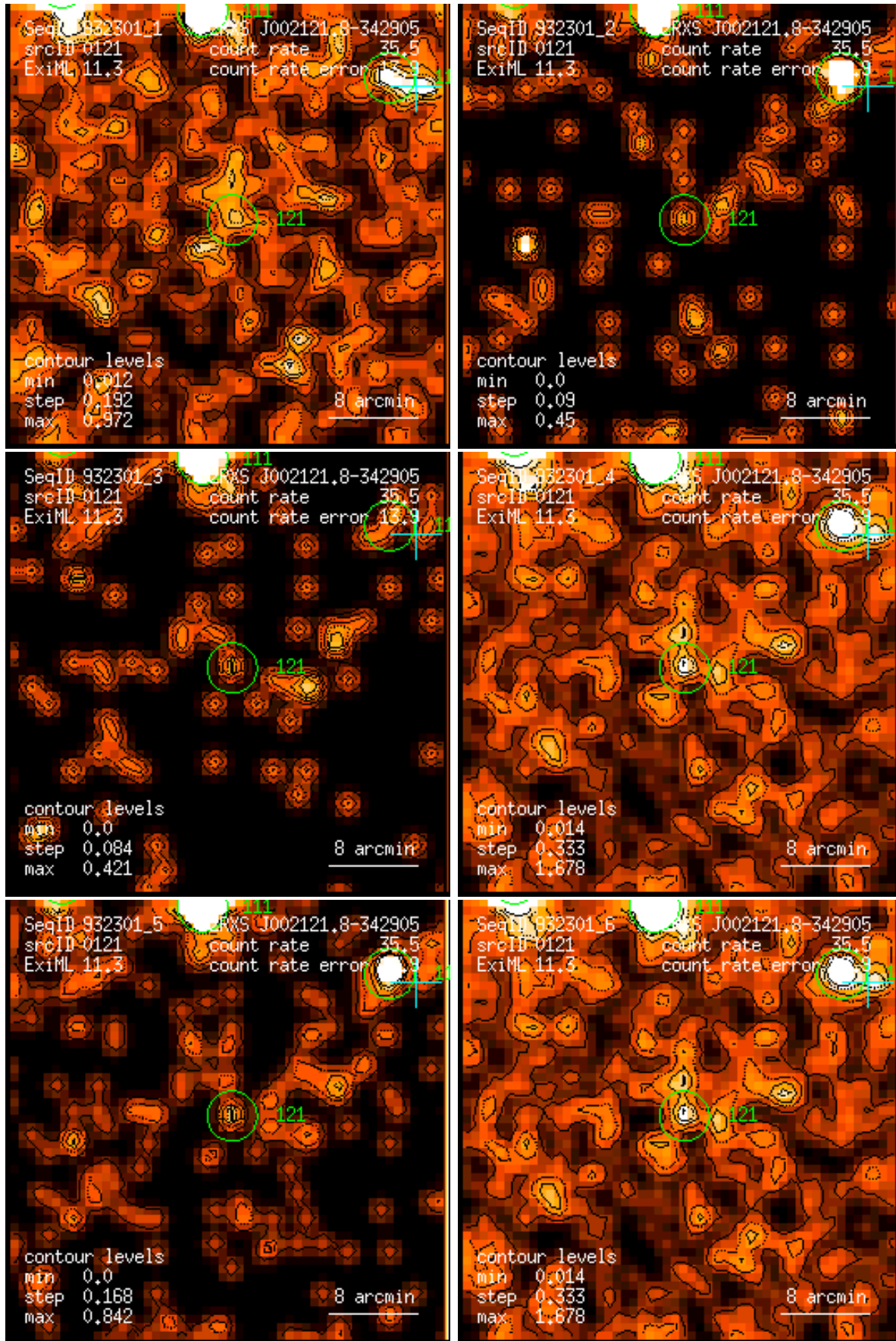
Figure 121: RASS 932301: detection 0121: band rate images, Gaussian filter: (1) PSPC channels 11 – 41, (2) 52 – 90, (3) 91 – 201, (4) 11 – 235, (5) 52 – 201, (6) 11 – 201. Broad band rates in counts/ks. Band rate contour levels in counts/ks/arcmin 2 .
