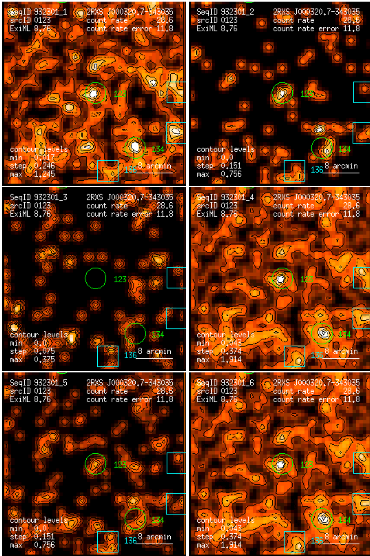
Figure 123: RASS 932301: detection 0123: band rate images, Gaussian filter: (1) PSPC channels 11 – 41, (2) 52 – 90, (3) 91 – 201, (4) 11 – 235, (5) 52 – 201, (6) 11 – 201. Broad band rates in counts/ks. Band rate contour levels in counts/ks/arcmin 2 .
