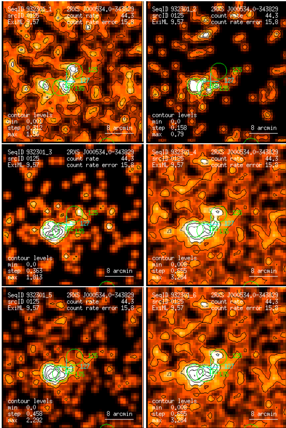
Figure 125: RASS 932301: detection 0125: band rate images, Gaussian filter: (1) PSPC channels 11 – 41, (2) 52 – 90, (3) 91 – 201, (4) 11 – 235, (5) 52 – 201, (6) 11 – 201. Broad band rates in counts/ks. Band rate contour levels in counts/ks/arcmin 2 .
