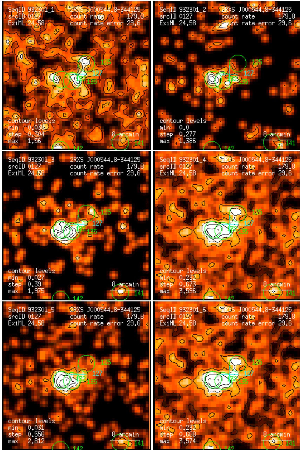
Figure 127: RASS 932301: detection 0127: band rate images, Gaussian filter: (1) PSPC channels 11 – 41, (2) 52 – 90, (3) 91 – 201, (4) 11 – 235, (5) 52 – 201, (6) 11 – 201. Broad band rates in counts/ks. Band rate contour levels in counts/ks/arcmin 2 .
