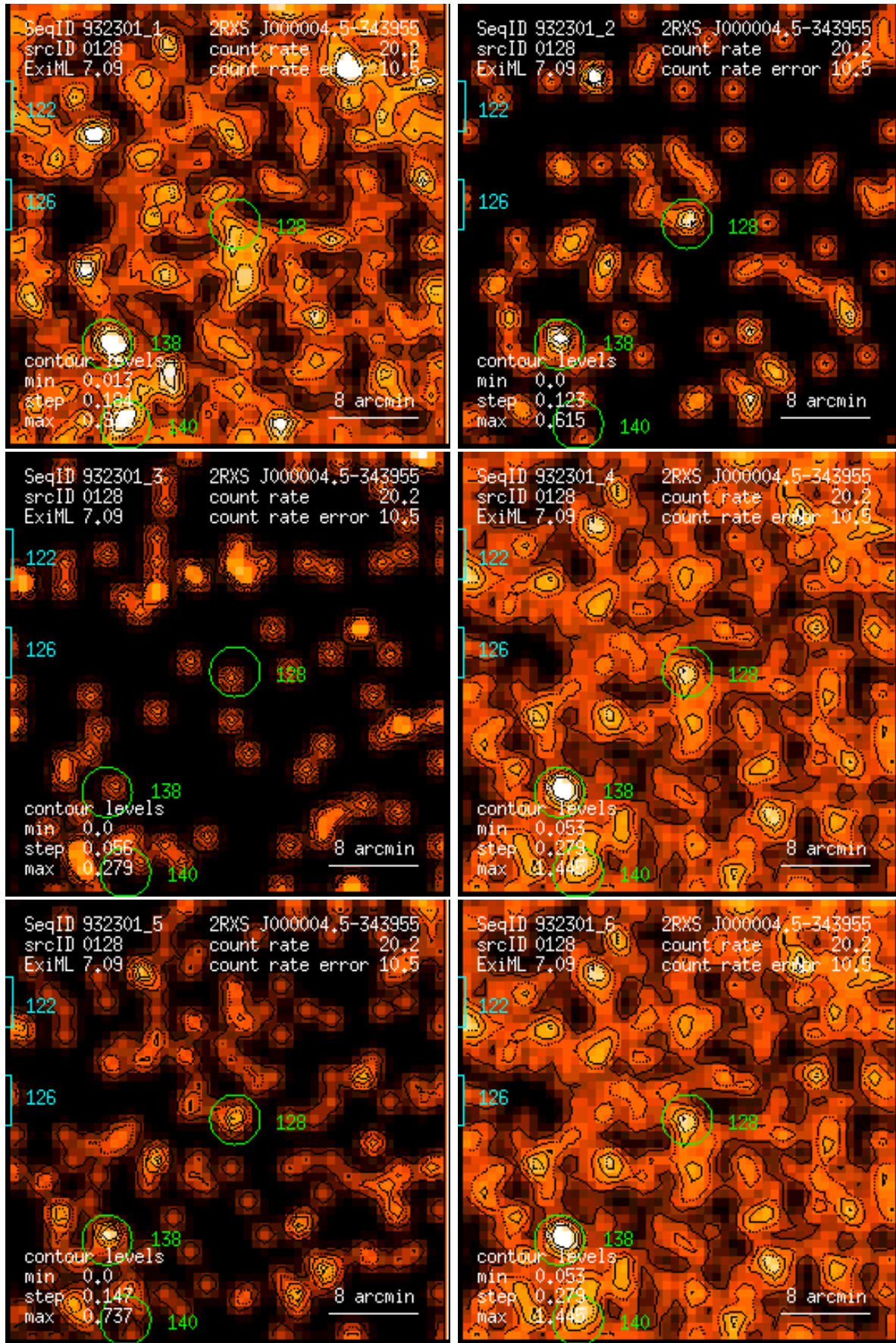
Figure 128: RASS 932301: detection 0128: band rate images, Gaussian filter: (1) PSPC channels 11 – 41, (2) 52 – 90, (3) 91 – 201, (4) 11 – 235, (5) 52 – 201, (6) 11 – 201. Broad band rates in counts/ks. Band rate contour levels in counts/ks/arcmin 2 .
