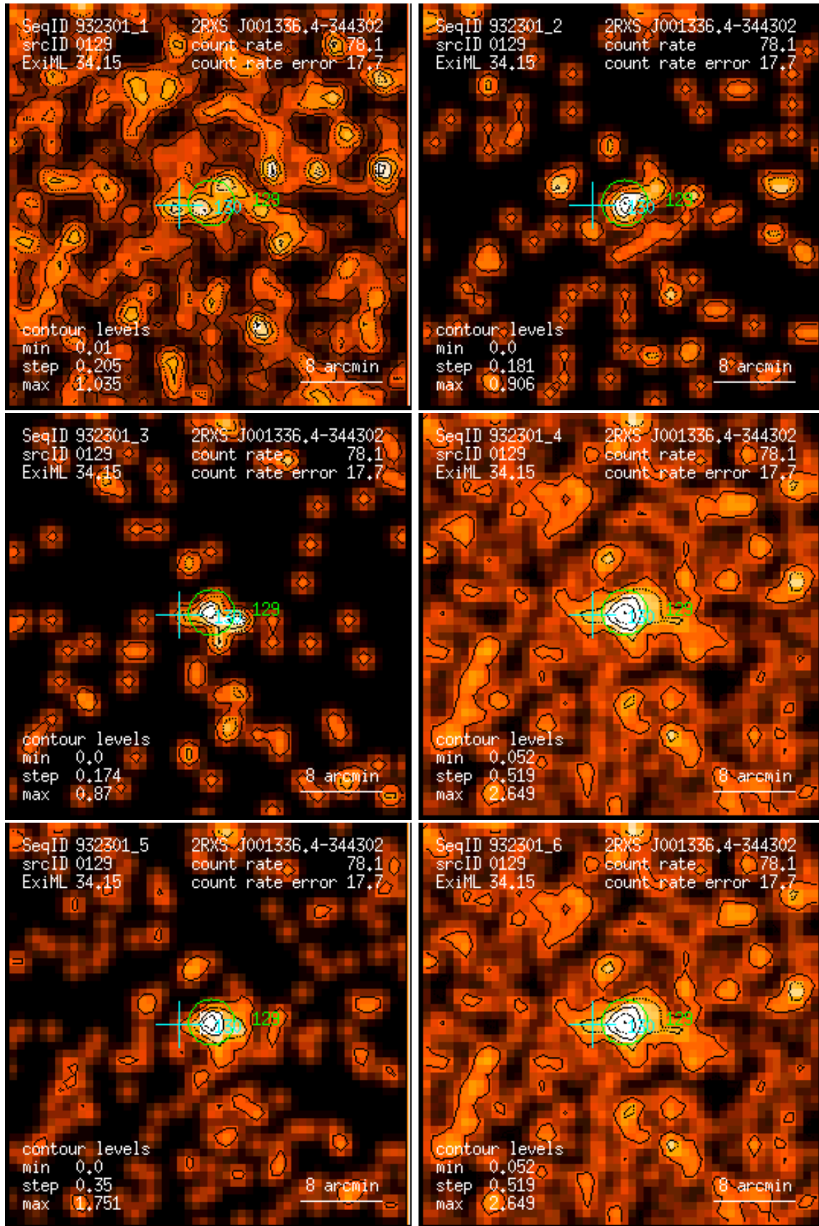
Figure 129: RASS 932301: detection 0129: band rate images, Gaussian filter: (1) PSPC channels 11 – 41, (2) 52 – 90, (3) 91 – 201, (4) 11 – 235, (5) 52 – 201, (6) 11 – 201. Broad band rates in counts/ks. Band rate contour levels in counts/ks/arcmin 2 .
