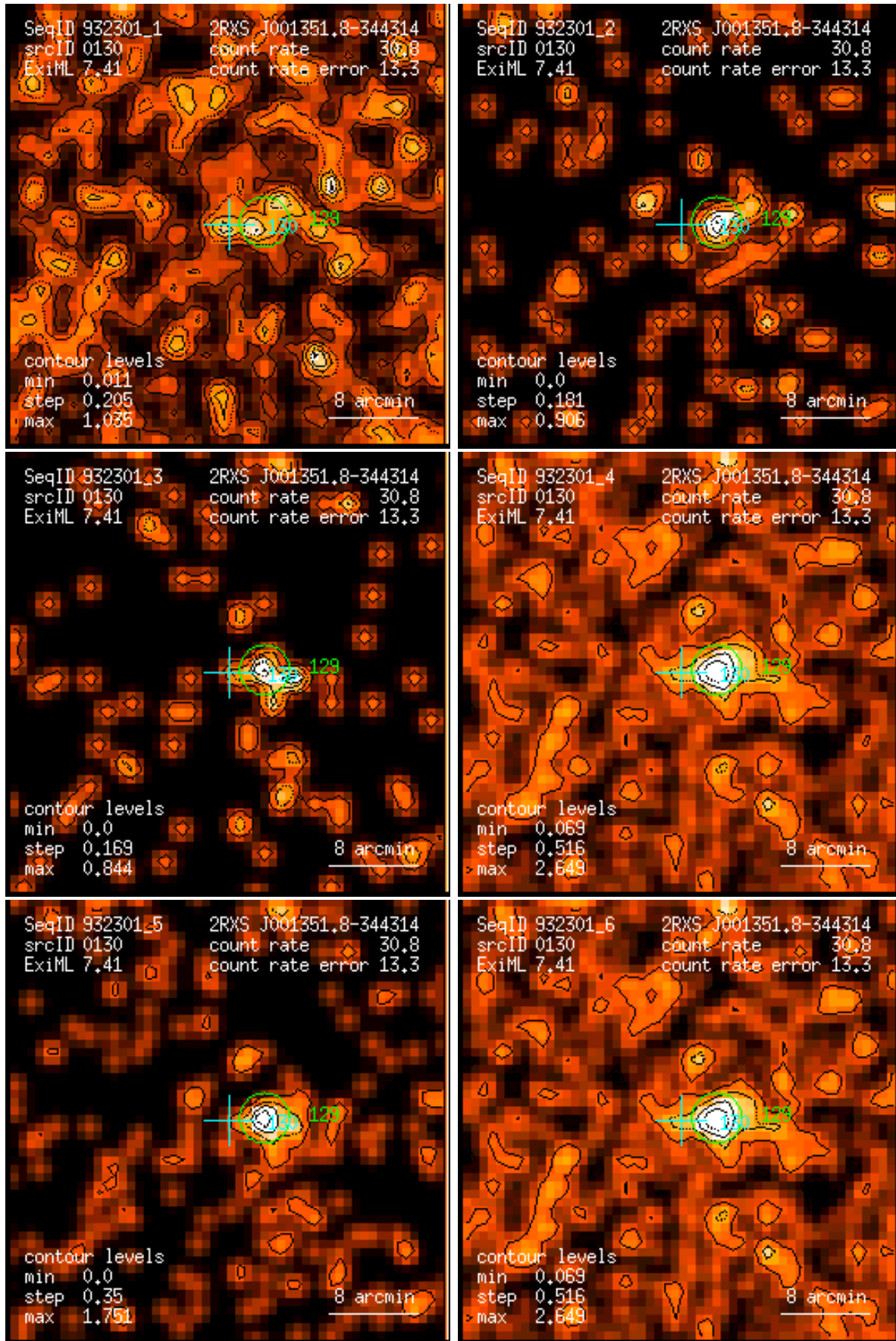
Figure 130: RASS 932301: detection 0130: band rate images, Gaussian filter: (1) PSPC channels 11 – 41, (2) 52 – 90, (3) 91 – 201, (4) 11 – 235, (5) 52 – 201, (6) 11 – 201. Broad band rates in counts/ks. Band rate contour levels in counts/ks/arcmin 2 .
