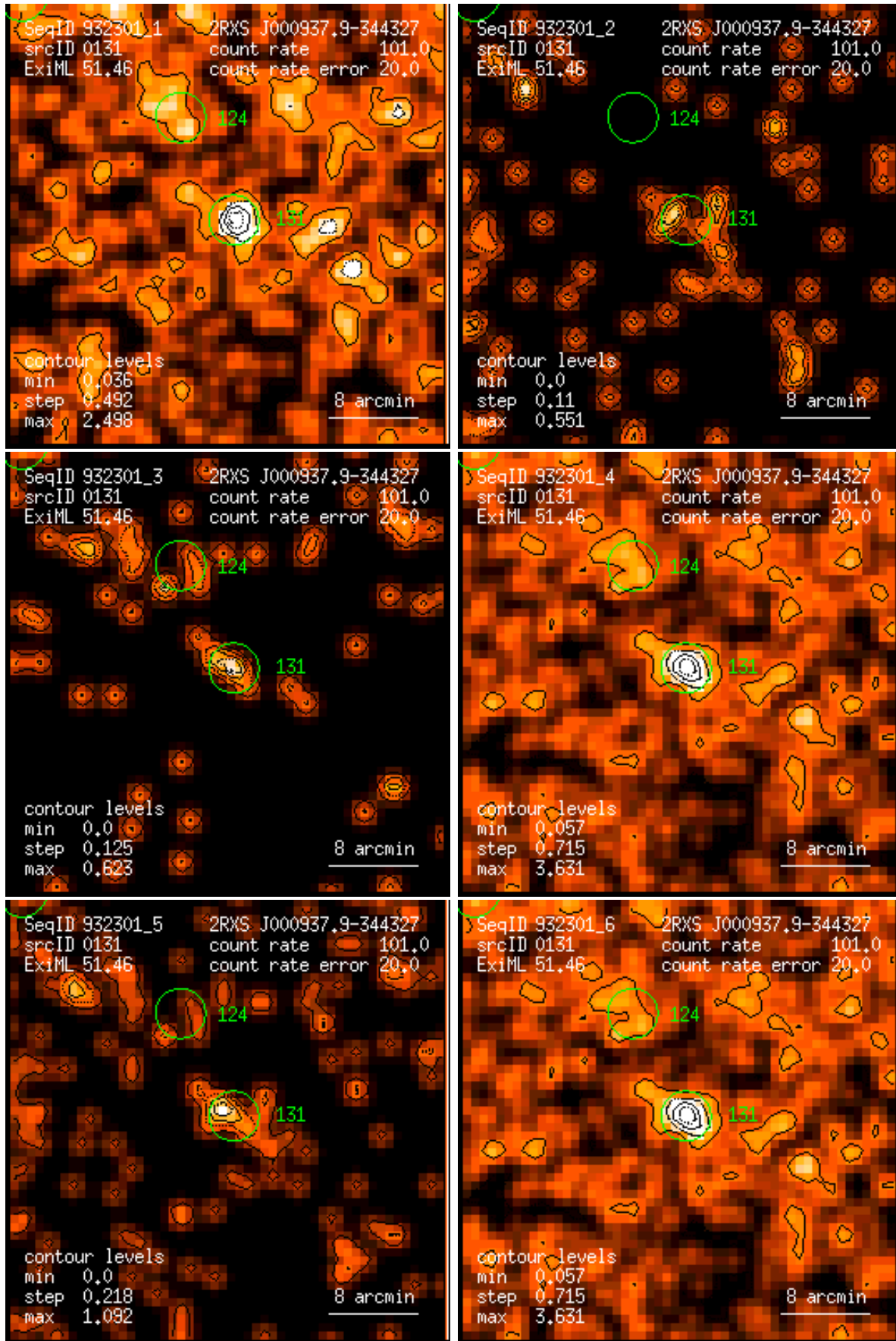
Figure 131: RASS 932301: detection 0131: band rate images, Gaussian filter: (1) PSPC channels 11 – 41, (2) 52 – 90, (3) 91 – 201, (4) 11 – 235, (5) 52 – 201, (6) 11 – 201. Broad band rates in counts/ks. Band rate contour levels in counts/ks/arcmin 2 .
