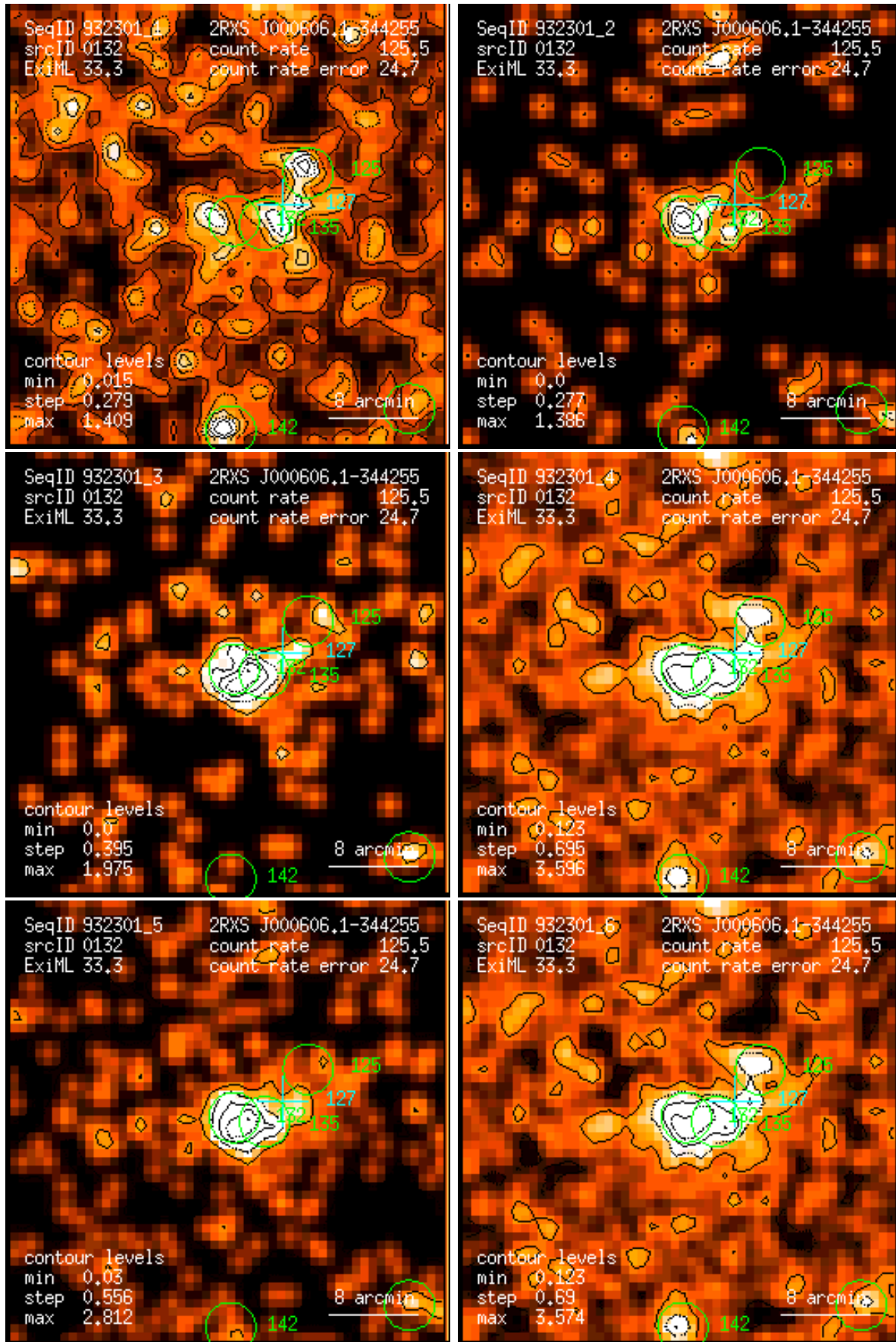
Figure 132: RASS 932301: detection 0132: band rate images, Gaussian filter: (1) PSPC channels 11 – 41, (2) 52 – 90, (3) 91 – 201, (4) 11 – 235, (5) 52 – 201, (6) 11 – 201. Broad band rates in counts/ks. Band rate contour levels in counts/ks/arcmin 2 .
